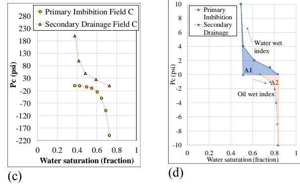
Figure 4. Capillary Pressure – primary imbibition and secondary drainage (a) Field A, (b) Field B and (c) Field C. (d)
