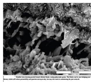
SEM – Glaucosite detailed view showing poorly chlorite blades coating glaucosite grains.
