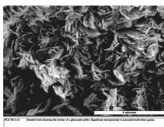
SEM – Glaucosite detailed view showing the texture of glaucosite pellets.
