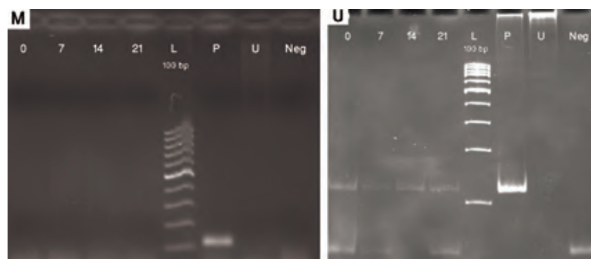
Fig.4: MSP results with methylated (M) and unmethylated (U) primers for BSP . Day 0; Undifferentiated MSCs, Days 7, 14 and 21; Osteoblastic differentiated cells days 7, 14, 21, respectively, P; Positive control (methylated and SBS treated DNA in M experiments and only SBS treated DNA in U experiments), U; SBS untreated DNA as negative control for MSP and Neg; No DNA as negative control. Amplicon size in BSP : M experiment (107 bp) and U experiment (110 bp). MSP; Methylation-specific PCR, BSP ; Bone sialoprotein , MSCs; Mesenchymal stem cells and SBS; Sodium bisulfite.
