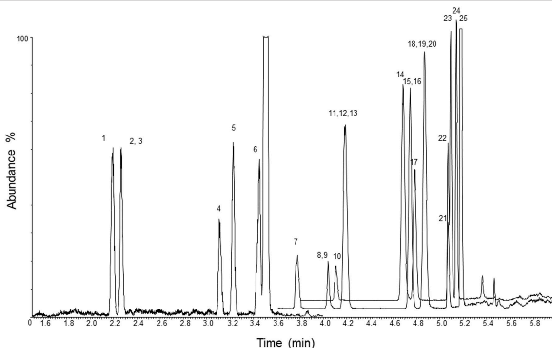
FIGURE 1 | LC-MS/MS chromatogram of a whole blood sample fortified with the analytes at the limit of quantification and their ISs. 1, methoxyacetyl norfentanyl; 2, acetyl norfentanyl; 3, acetyl norfentanyl-D5; 4, norfentanyl; 5, furanyl norfentanyl; 6, cyclopropyl norfentanyl; 7, butyryl norfentanyl; 8, butyrylfentanyl carboxy metabolite; 9, methoxyacetylfentanyl; 10, \beta -hydroxythiofentanyl; 11, valerylfentanyl carboxy metabolite; 12, furanylethyl fentanyl; 13, acetylfentanyl; 14, fentanyl; 15, fentanyl-D5; 16, despropionylfentanyl (4-ANPP); 17, alfentanil; 18, furanylfentanyl; 19, despropionyl para -fluorofentanyl; 20, cyclopropylfentanyl; 21, carfentanil; 22, butyrylfentanyl; 23, sufentanil; 24, \beta -hydroxyfentanyl; 25, phenylacetyl fentanyl.
