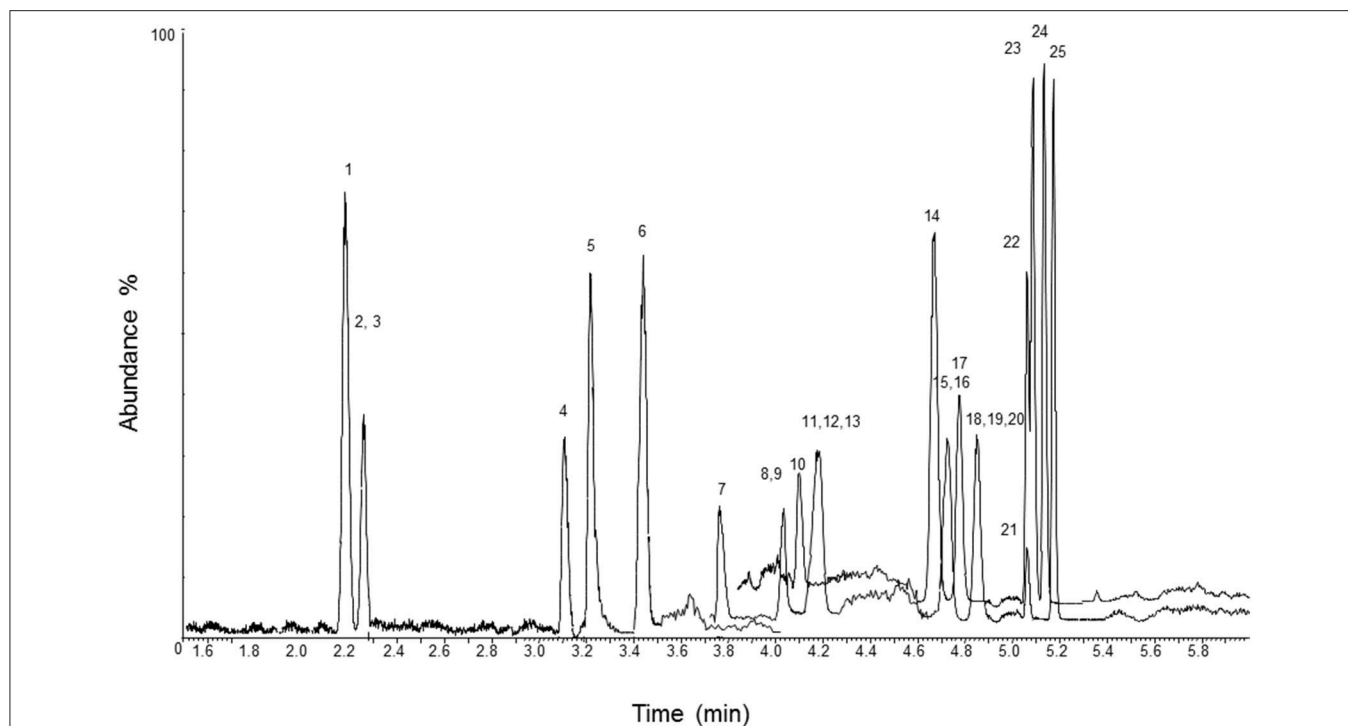
FIGURE 2 | LC-MS/MS chromatogram of a urine sample fortified with the analytes at the limit of quantification and their ISs. 1, methoxyacetyl norfentanyl; 2, acetyl norfentanyl; 3, acetyl norfentanyl-D5; 4, norfentanyl; 5, furanyl norfentanyl; 6, cyclopropyl norfentanyl; 7, butyryl norfentanyl; 8, butyrylfentanyl carboxy metabolite; 9, methoxyacetylfentanyl; 10, \beta -hydroxythiofentanyl; 11, valerylfentanyl carboxy metabolite; 12, furanylethyl fentanyl; 13, acetylfentanyl; 14, fentanyl; 15, fentanyl-D5; 16, despropionylfentanyl (4-ANPP); 17, alfentanil; 18, furanylfentanyl; 19, despropionyl para -fluorofentanyl; 20, cyclopropylfentanyl; 21, carfentanil; 22, butyrylfentanyl; 23, sufentanil; 24, \beta -hydroxyfentanyl; 25, phenylacetyl fentanyl.
