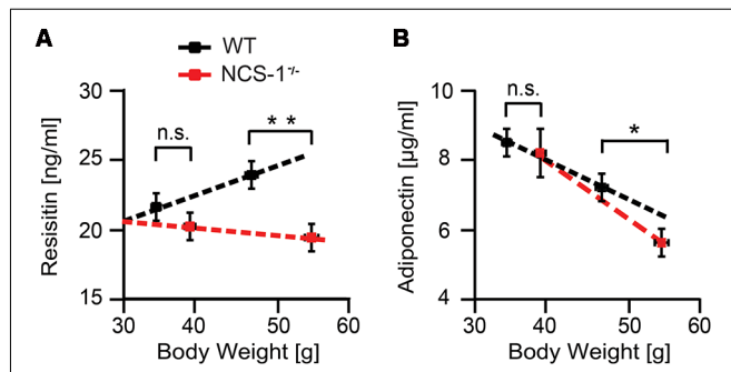
FIGURE 4 | Reduced concentrations of resistin and adiponectin in NCS-1 -/- serum. (A) Relation between resistin serum concentration and body weight for 25-week-old NCS-1 -/- mice ( n = 8–10) and WT littermates ( n = 8–10). (B) Relation between adiponectin concentration and body weight for 25-week-old NCS-1 -/- mice ( n = 8) or WT littermates ( n = 10). Mice were kept either on normal chow ( n = 10) or fed HFD after week 6 ( n = 8). Bars represent mean values \pm SEM. n.s.—not significant; * P < 0.05; ** P < 0.01 (MANOVA and Bonferroni post hoc test).
