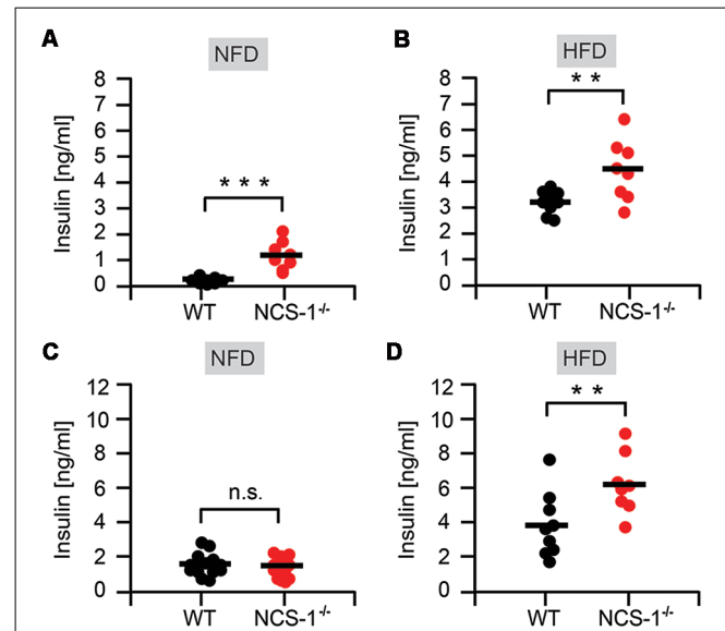
FIGURE 3 | Hyperinsulinemia in NCS-1 -/- mice. (A) Plasma insulin concentration in 20-week-old WT and NCS-1 -/- mice fed normal chow (NFD) and fasted for 16 h. (B) Plasma insulin concentration in 20-week-old WT and NCS-1 -/- mice fed HFD and fasted for 16 h. (C) Plasma insulin concentration in glucose tolerance test. WT- and NCS-1 -/- -mice fed normal chow (NFD) and fasted, were injected intraperitoneally with 2 mg glucose/g body mass. Plasma insulin concentrations were determined 30 min later. (D) WT- and NCS-1 -/- -mice fed HFD and fasted, were injected intraperitoneally with 2 mg glucose/g body mass. Plasma insulin concentrations were determined 30 min later. Values are presented as mean ± SEM. n.s.—not significant; ** P < 0.01 ; *** P < 0.001 (MANOVA and Bonferroni post hoc test).
