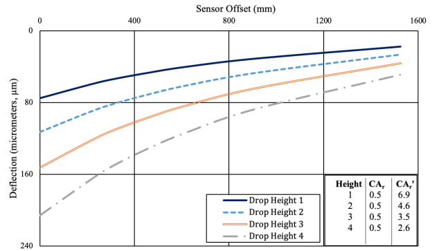
Fig. 2. Illustration on importance of CA_r' based on SHRP section 1049.
