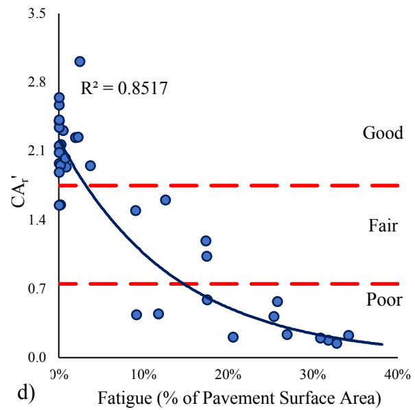
Fig. 3. Development of CA_r' scale to rank pavement sections based on fatigue: (a) drop height 1, (b) drop height 2, (c) drop height 3, and (d) drop height 4.
