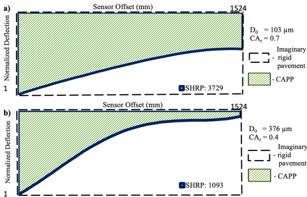
Fig. 1. Normalized area of deflection profiles for SHRP sections: (a) 3729 and (b) 1093.
