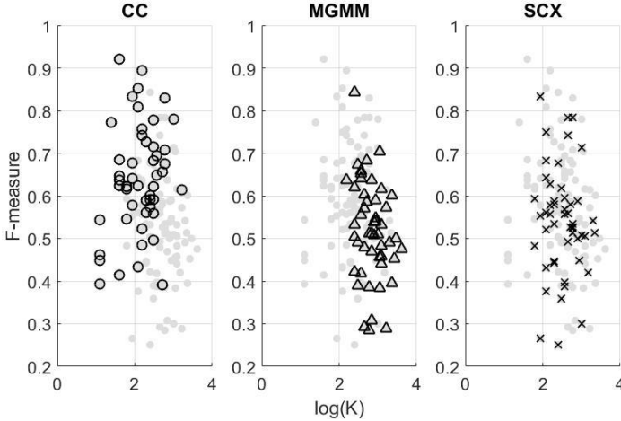
Fig. 3. Number of keyframes (K) and F-measure averaged over five user ground-truths, for summaries of the 50 VSUMM videos. Filled, grey circles show the results for all three methods, with the points for the named method highlighted in black.
