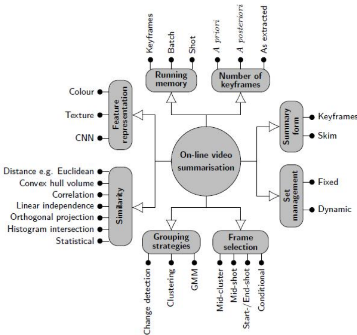
Fig. 1. A classification of on-line video summarisation methods.
