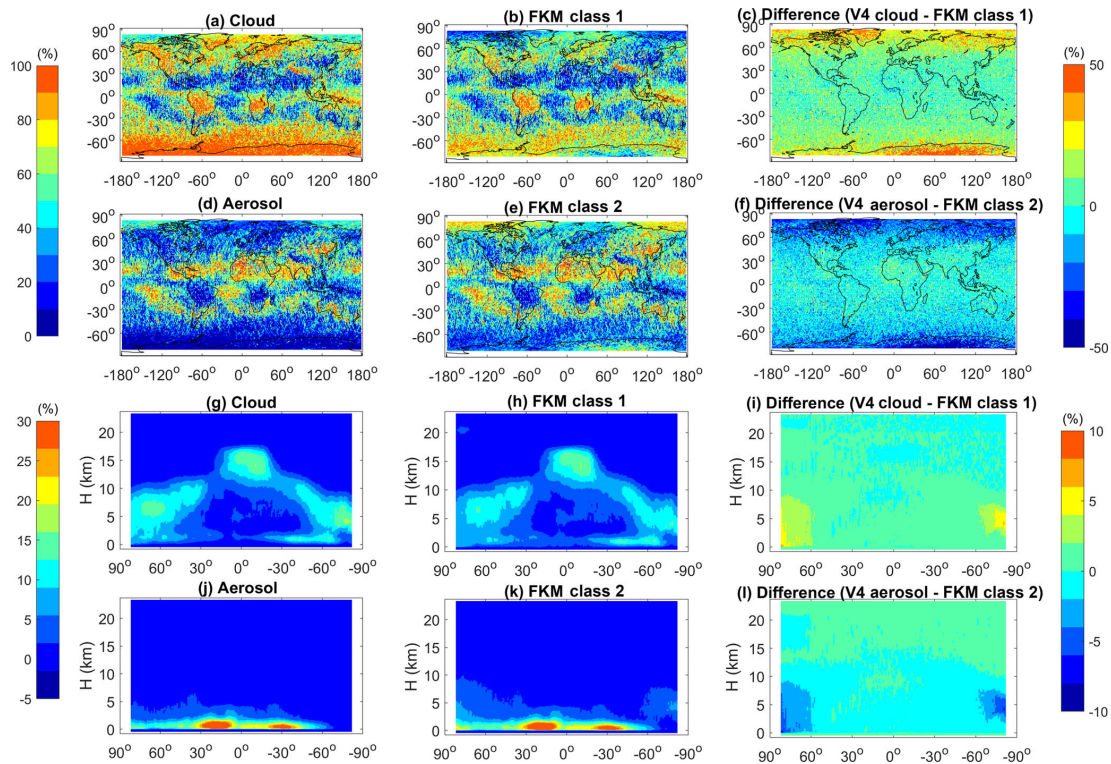
Figure 7. Distributions of feature type occurrence frequencies during January 2008. Panels in the left column show V4 COCA results; panels in the center column show CAD FKM two-class results; and the panels in the right column show the percentages of differences between the left and center columns. The top two rows show maps of occurrence frequencies as a function of latitude and longitude for clouds (a–c) and aerosols (d–f). The bottom two rows show the zonal mean occurrence frequencies of clouds (g–i) and aerosols (j–l).
