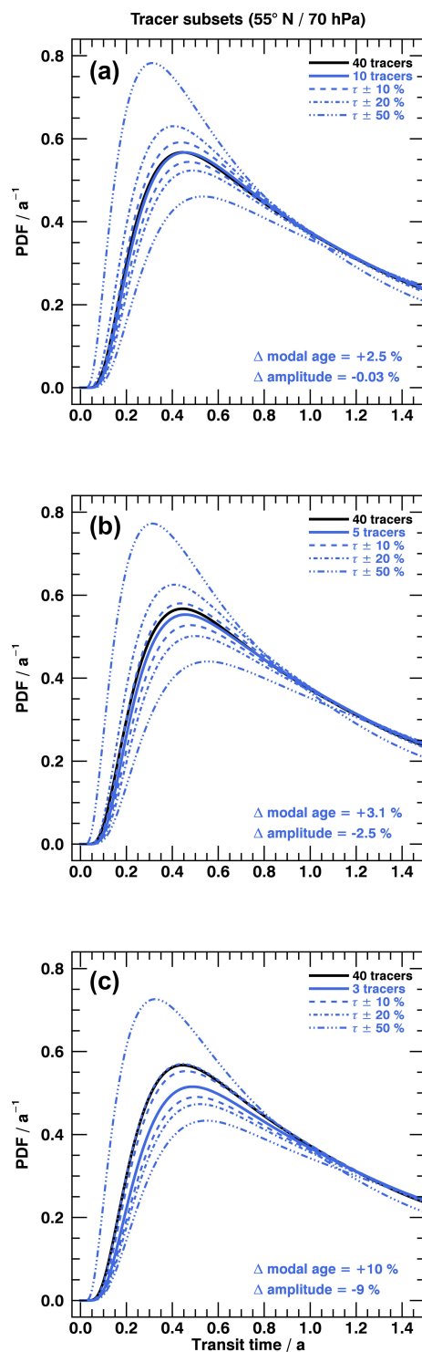
Figure 12. Annual mean age spectra from radioactive tracer subsets compared to full set at 55^\circ\text{N} and 70\text{ hPa} . The black solid line corresponds to the full set (40 tracers), while the solid blue line denotes spectra of a subset with 10 tracers (a), 5 tracers (b) and 3 tracers (c). The changes in modal age and amplitude for the solid blue lines relative to the black lines are given in each panel in the bottom right corner. The three dashed and dashed–dotted spectra in each panel include an error in the knowledge of the local chemical lifetimes of \pm 10\% , \pm 20\% and \pm 50\% (see text for details).
