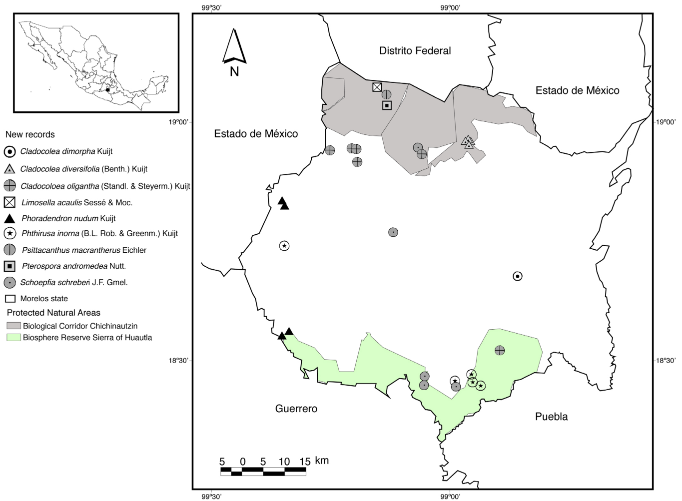
Figure 1. Map of Morelos state, Mexico, showing the Natural Protected Areas where new flowering plant records occur. Symbols indicate each species.
