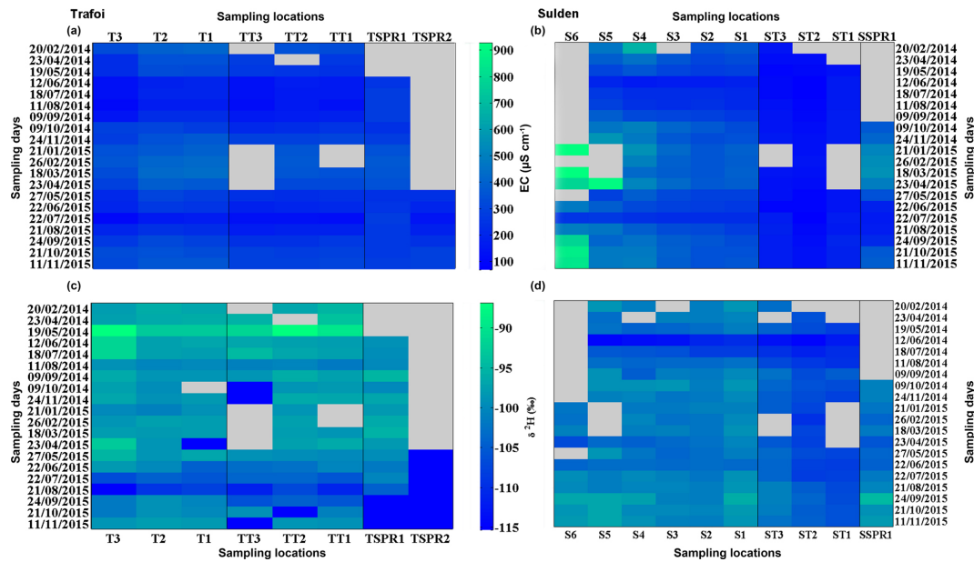
Figure 4. Spatial and temporal variability in EC ( \mu\text{S cm}^{-1} ) and \delta^{2}\text{H} (‰) at different stream sections, tributaries and springs within the Trafoi sub-catchment (a, c) and the Sulden sub-catchment (b, d) in 2014 and 2015. The heat maps are grouped into locations at streams, tributaries and springs. Grey areas refer to missing sample values due to frozen or dried-out streams or tributaries or because the sampling location was included later in the sampling scheme.
