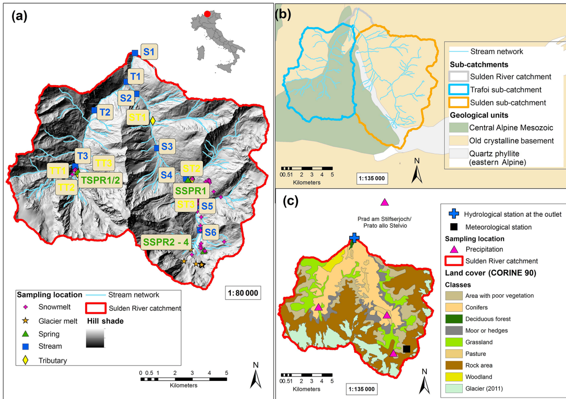
Figure 1. Overview of the Sulden catchment with (a) sampling points, (b) geology and (c) land cover with instrumentation. The meteorological station shown is the Madritsch (Madriccio) AWS of the Hydrographic Office (Autonomous Province of Bozen-Bolzano). The glacier extent of 2011 is based on Smiraglia (2015).
