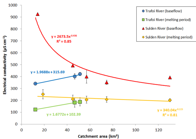
Figure 5. Spatial variability in electrical conductivity along the Trafoi and Sulden River against catchment area. Electrical conductivity is averaged for sampling days during baseflow conditions (21 January, 26 February and 18 March 2015) and melting period (12 June, 18 July, 11 August and 9 September 2014).
