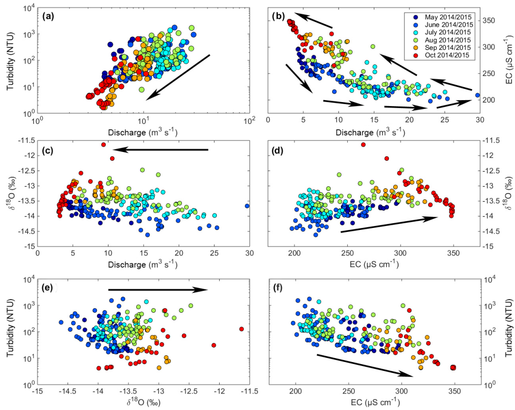
Figure 9. Monthly relationships between (a–e) discharge, turbidity and tracers such as EC and \delta^{18}\text{O} at the outlet Stilfserbrücke in 2014 and 2015. The dataset consists of n = 309 samples. Arrows underline the monthly pattern.
