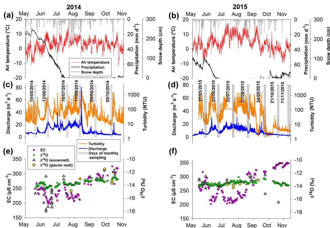
Figure 8. Time series from 2014 and 2015 of (a, b) precipitation, hourly air temperature and snow depth at the AWS Madritsch; (c, d) streamflow and turbidity; and (e, f) electrical conductivity and \delta^{18}\text{O} of the stream at the outlet Stilfserbrücke and of snowmelt and glacier meltwater. Grey shaded bars indicate the date of monthly sampling carried out in the entire catchment.
