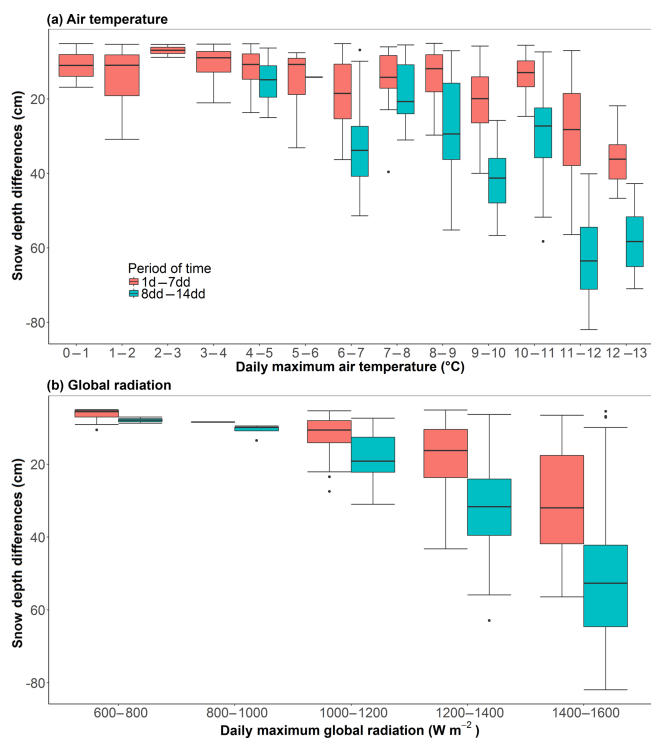
Figure 6. Box plots of environmental variables (a) daily maximum air temperature and (b) daily maximum global radiation on snowmelt expressed as snow depth differences at AWS Madritsch. Snow depth differences smaller than 5 cm are discarded from analysis. dd refers to the days considered for analysis.
