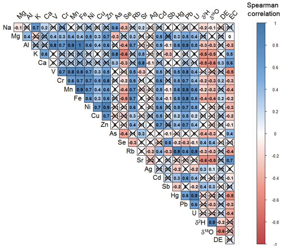
Figure 3. Spearman's rank correlation matrix of hydrochemical variables. Values are shown for a level of significance p < 0.05 , and otherwise crossed out.
