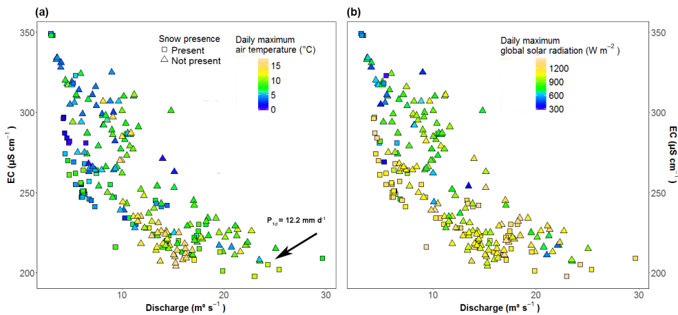
Figure 10. Monthly relationships between discharge and electrical conductivity (EC) at the outlet Stilfserbrücke with respect to (a) daily maximum air temperature (1 d) and (b) daily maximum global solar radiation (1 d) compared to the snow presence measured at the AWS Madritsch in 2014 and 2015. Different symbols indicate the snow presence. The arrow indicates a storm event.
