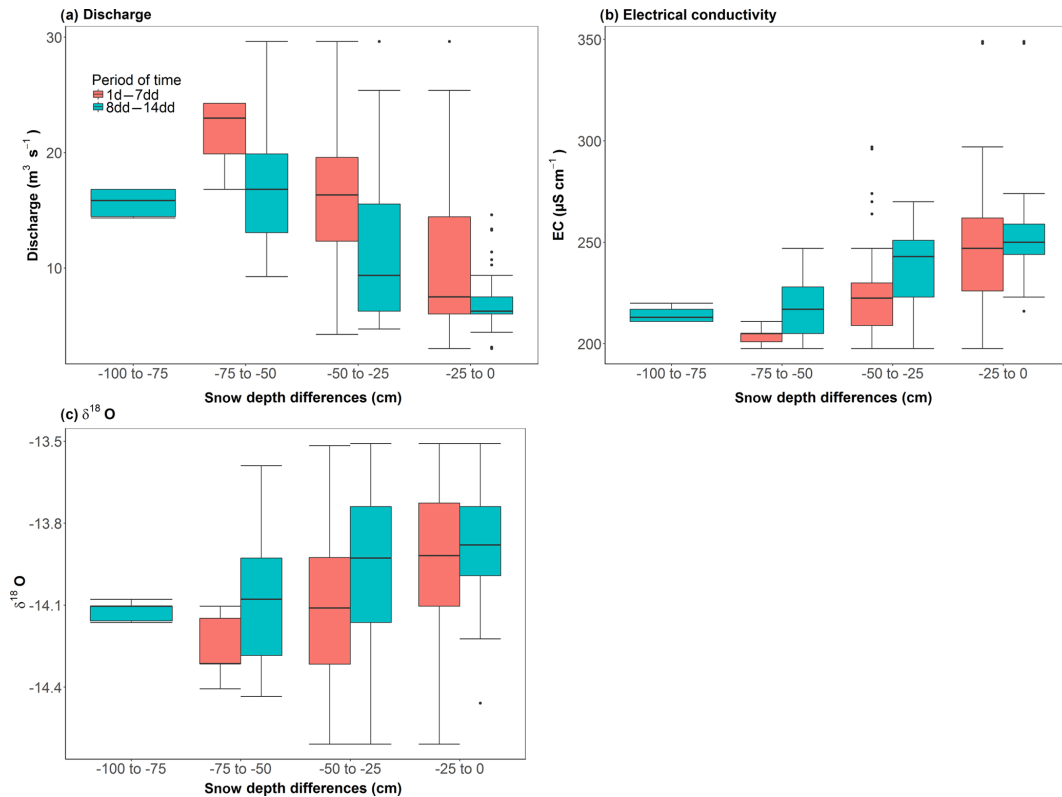
Figure 7. Box plots of snowmelt expressed as snow depth differences at AWS Madritsch on the variability in (a) discharge, (b) EC and (c) \delta^{18}\text{O} at the outlet Stilfserbrücke in 2014 and 2015. dd refers to the days considered for analysis.
