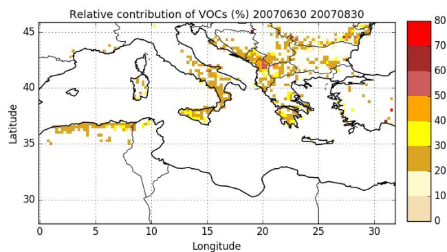
Figure 8. Relative contribution of VOCs to gaseous precursors (VOCs plus gaseous I/S/L-VOCs; %) emitted by wildfires over the Mediterranean area during the summer of 2007.
