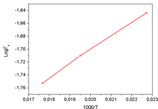
Fig. 5. Temperature dependence of the change in the deuterium solubility coefficient for palladium-silver filter.
