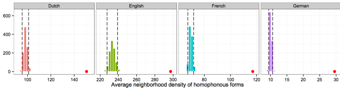
Figure 13. Average neighborhood density among all homophonous forms (red dots) compared to the chance level (histograms). In all 4 languages, the average neighborhood density of homophones is higher than what would be expected by chance.
