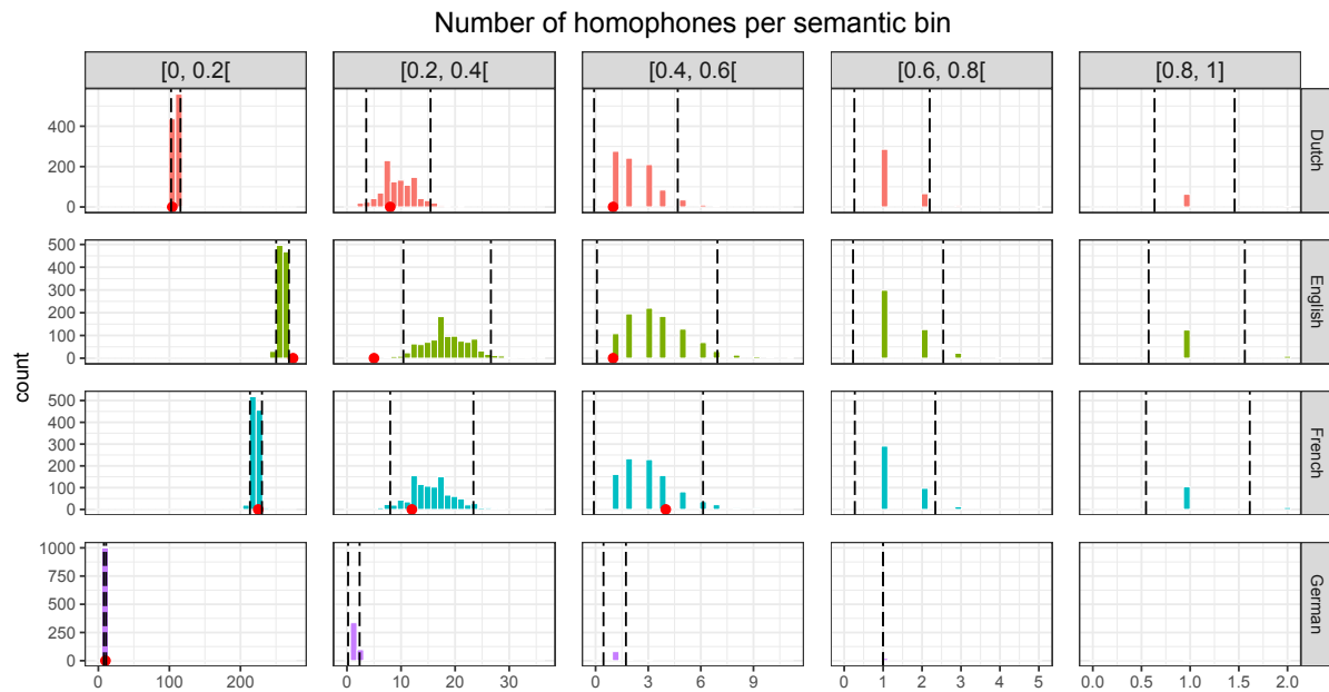
Figure 11. Number of homophone pairs per semantic bin. The histograms show the number of pairs of homophones found in the random baselines for each 0.2 bin of cosine value compared to the number of pairs of homophones in the lexicons (red dots) in the same bin. There is no pair of homophone in the bins that capture the most similar words (values close to 1, rightmost graphs), despite the fact that the random baselines span the full range of cosine values.
