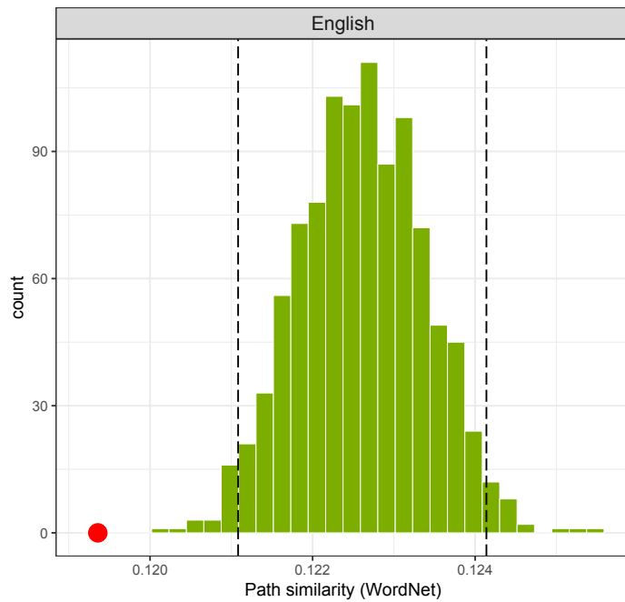
Figure S5. The histogram shows the distribution of the average semantic distance (computed using WordNet) between members of a pair of homophones in our random baselines compared to the English lexicon (the red dot). The dotted lines represent 95% confidence intervals derived from the distribution of random baselines. Homophones are more semantically distant in English than expected by chance.
