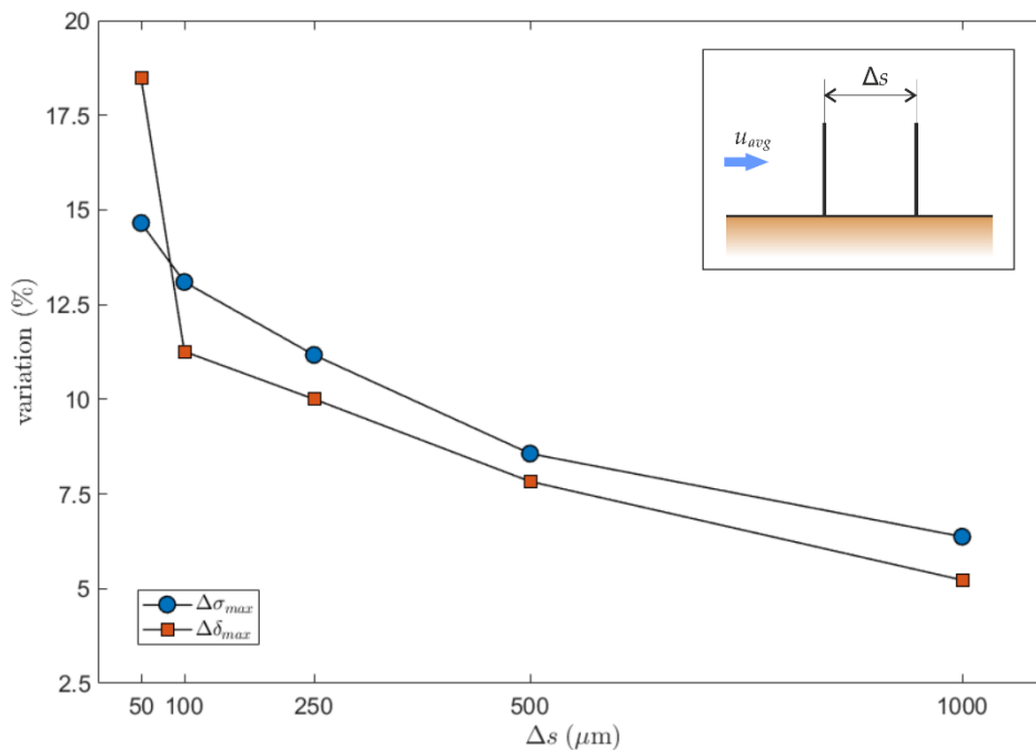
Fig. 3. Difference on the maximum von Mises stress and the maximum displacement between the first and the second hair as function of the hair spacing. Inset: schematic view of the considered geometry.
