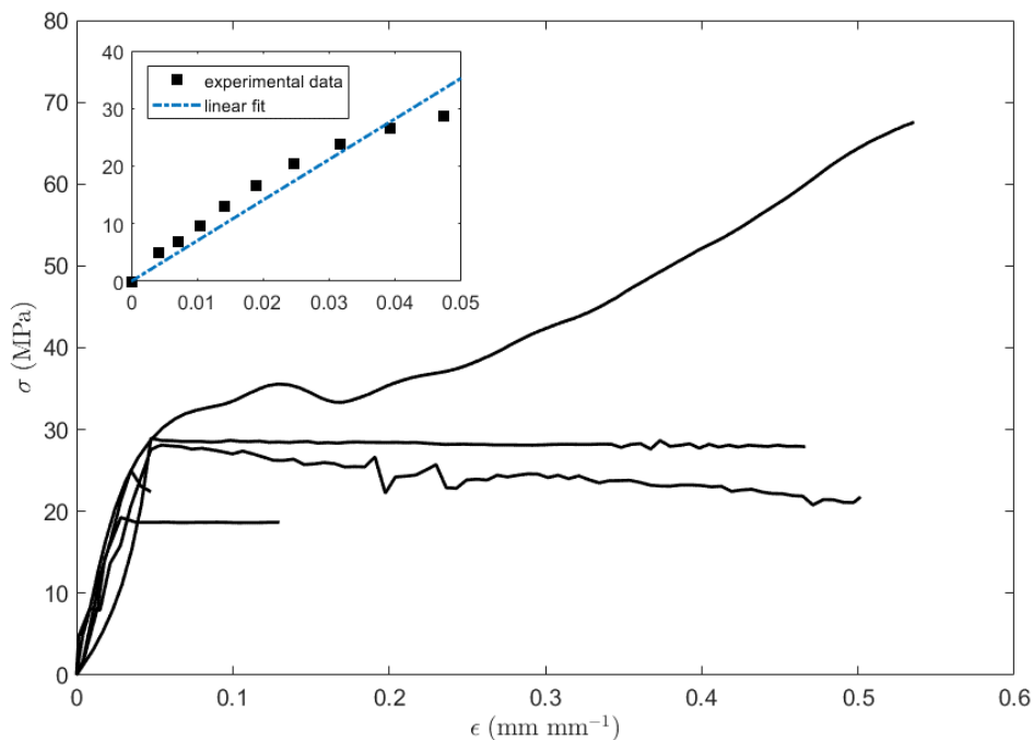
Fig. A1. Example stress-strain curves of different Theraphosa stirmi 's hairs obtained through nanotensile tests. Inset: example linear fit on the first part of a curve, with extracted Young's modulus E \approx 705.8 MPa ( R^2 -value = 0.921).
