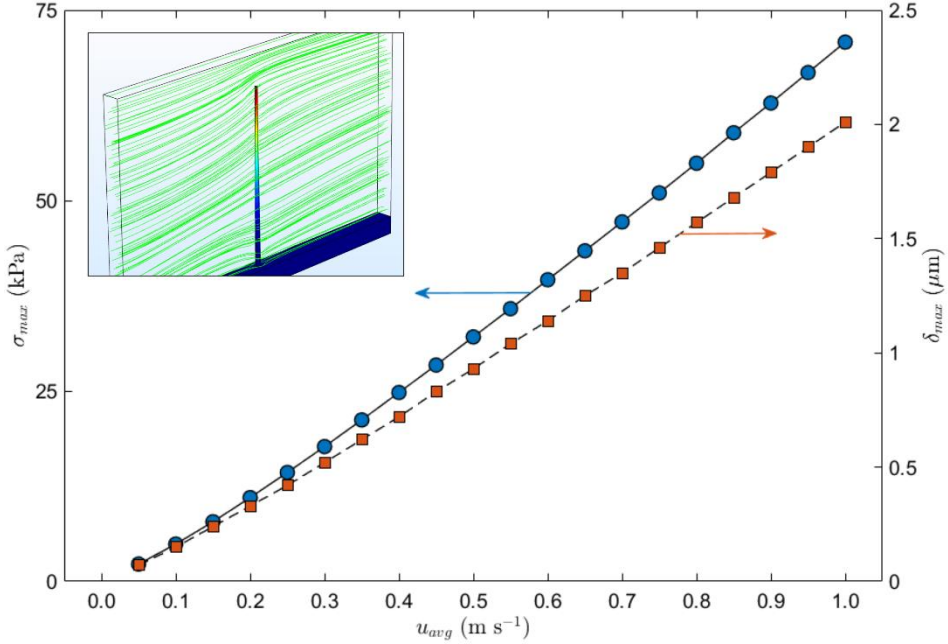
Fig. 2. Maximum von Mises stress and maximum hair displacement as function of the mean inlet velocity. Inset: qualitative visualization of the displacement field of the structure and of the flow streamlines.
