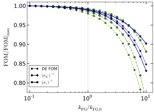
FIG. 24.— The effect of rescaling the foreground cutoff scale, k_{\text{FG}} , on the normalised FOM/marginal errors (see Fig. 21 for key). The base value of the cut-off scale is k_{\text{FG},0} = 2\pi/(r\nu\Delta\bar{\nu}_{\text{tot}}) .
