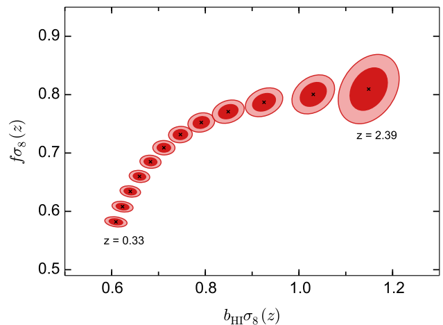
FIG. 10.— Constraints on b_{\text{HI}}\sigma_8 and f\sigma_8 as a function of redshift, for the Facility survey.
