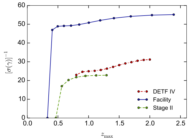
FIG. 18.— Improvement in \gamma constraints a function of maximum redshift of the survey. We have marginalised over w_0 , w_a and \Omega_K here. The low value in the first redshift bin for the IM experiments is due to a degeneracy.
