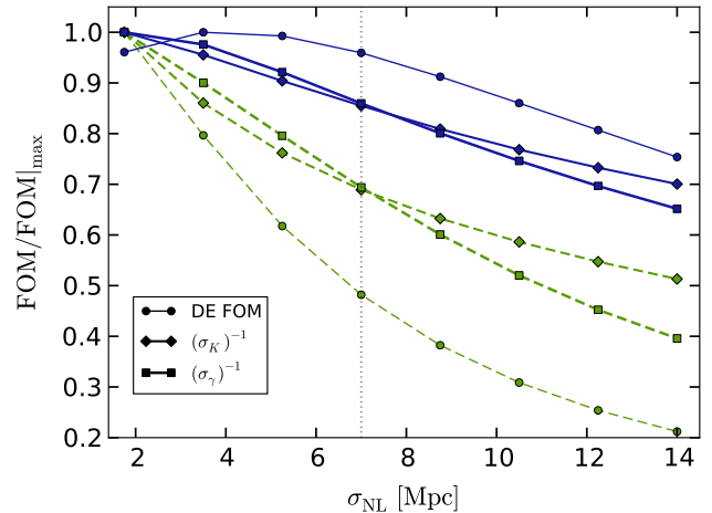
FIG. 22.— Normalised FOM/marginal errors as a function of \sigma_{\text{NL}} (see Fig. 21 for key).
