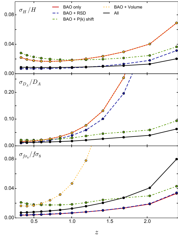
FIG. 8.— Fractional errors on H(z) , D_A(z) , and f\sigma_8(z) for the Facility experiment, for various combinations of distance terms being switched on and off in the Fisher matrix calculation. The RSDs are taken to include both the angle-dependence and non-linear cut-off terms (see text).
