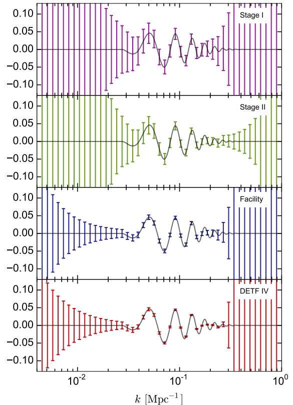
FIG. 5.— Forecast constraints on the BAO wiggles, combined over the whole redshift range for each of the reference surveys.
