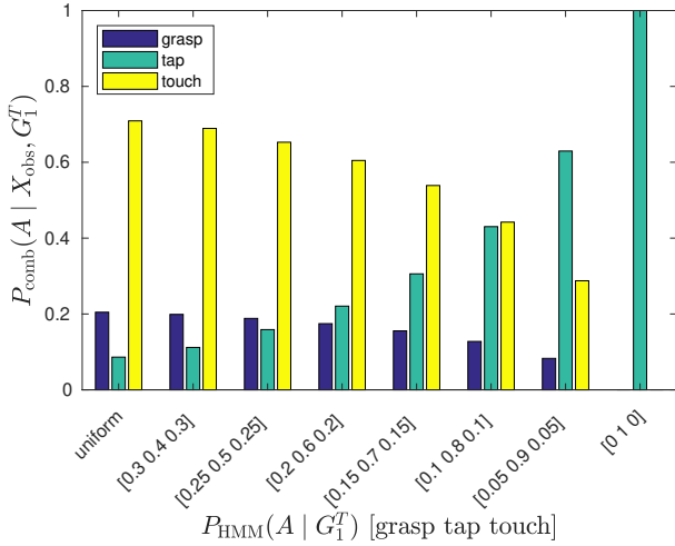
Figure 3: Inference over action given the evidence X_{\text{obs}} = \{\text{Size} = \text{small}, \text{Shape} = \text{sphere}, \text{ObjVel} = \text{slow}\} , combined with different probabilistic soft evidence about the action.
