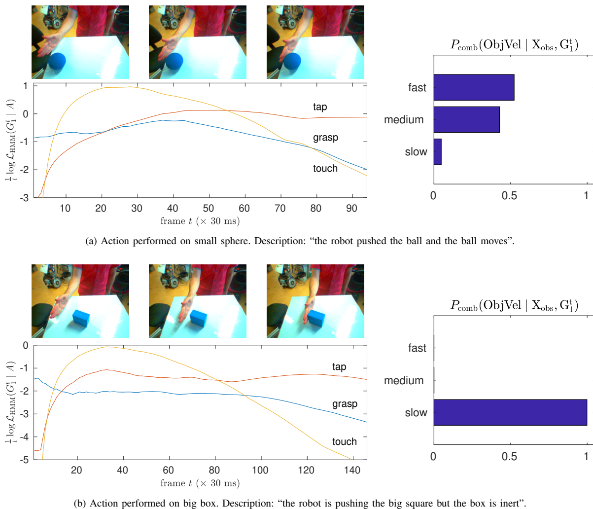
Figure 5: Object velocity effect anticipation before impact. The evidence from the gesture recognizer (left) is fed into the Affordance–Words model before the end of the execution. The combined model predicts the effect (right) and describes it in words.
