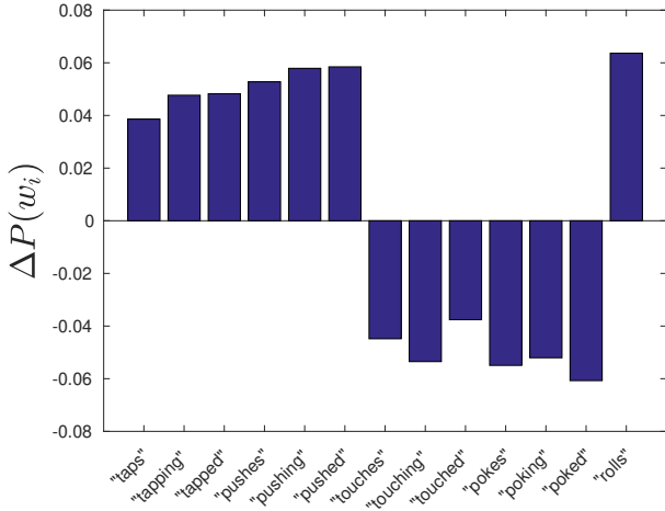
Figure 6: Variation of word occurrence probabilities: \Delta P(w_i) = P_{\text{comb}}(w_i | X_{\text{obs}}, \text{Action}=\text{tap}) - P_{\text{BN}}(w_i | X_{\text{obs}}) , where X_{\text{obs}} = \{\text{Size}=\text{big}, \text{Shape}=\text{sphere}, \text{ObjVel}=\text{fast}\} . This variation corresponds to the difference of word probability when we add the tap action evidence (obtained from gesture recognition) to the initial evidence about object features and effects. We have omitted words for which no significant variation was observed.
