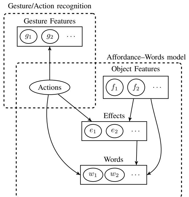
Figure 2: Abstract representation of the probabilistic dependencies in the model.
