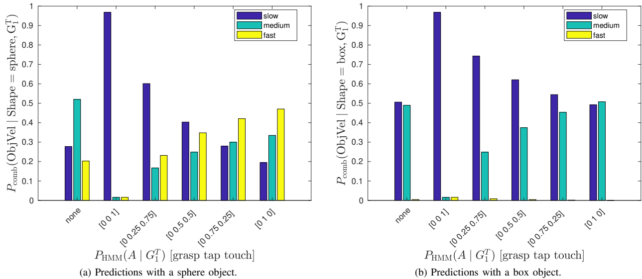
Figure 4: Inference over the object velocity effect of different objects, when given probabilistic soft evidence about the action.
