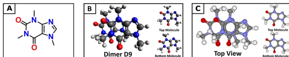
Fig. 1 A) The skeletal chemical structure of caffeine. B) The most stable dimer structure (D9) in water as calculated using the proposed computational approach. C) The dimer structure of caffeine as found in the solid state. 67,68 For clarity the reciprocal orientations of the top and bottom molecules in the dimer in (B) and (C) are reported separately.
