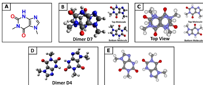
Fig. 3 A) The skeletal chemical structure of paraxanthine. B) Stable dimer structure in gas phase as calculated using the proposed computational approach. C) The \pi - \pi stacking dimer synthon of paraxanthine as found in X-Ray structure. For the dimer structures (B, C) the top and bottom molecules are reported separately to clarify the reciprocal orientation. D) Stable dimer structure linked by H-bond interactions as calculated using the proposed computational approach. E) The later dimer synthon of paraxanthine as found in X-Ray structure.
