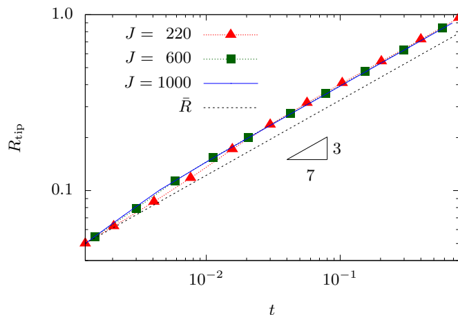
FIG. 4. Log-log plot of R_{\text{tip}} as a function of time a for J = 220, 600 and 1000 . In each case, the interface is initially perturbed by the single, most-rapidly growing mode. The dotted line shows the radius of the axisymmetrically growing bubble, \bar{R}(t) .
