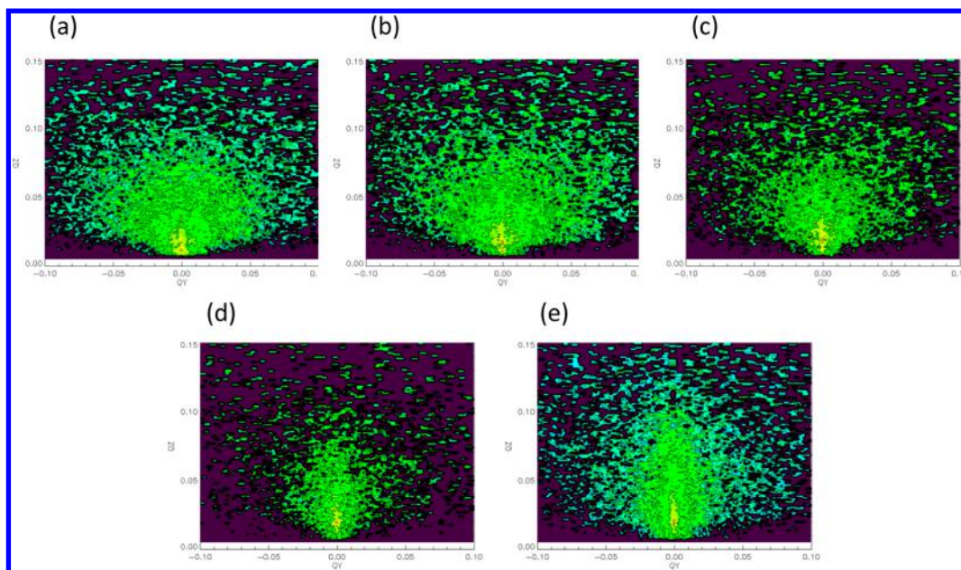
Figure 3. GISANS data from a 1 wt % solution of RFL 4 FR at rest or under steady shear (a) at rest (following shear at 1000 s -1 ), (b) 0.01 s -1 , (c) 1 s -1 , (d) 100 s -1 , (e) 1000 s -1 . The QZ axis is along the shear gradient, and the QY direction is mainly oriented along the shear flow. The axis units are in Å -1 . The intensity is plotted on a logarithmic color scale.
