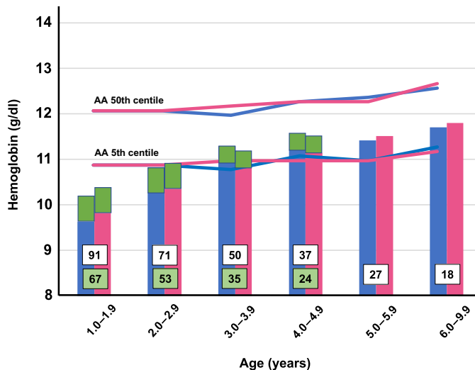
Fig. 3. Hb levels in rural Gambian children compared to U.S. reference data for African Americans. Mean Hb levels from healthy rural Gambian children participating in the Keneba Biobank compared to reference data from African Americans (AA) living in the United States (24). Blue, boys; pink, girls. 1 to 1.99 years, n = 344 ; 2 to 2.99 years, n = 563 ; 3 to 3.99 years, n = 518 ; 4 to 4.99 years, n = 495 ; 5 to 5.99 years, n = 446 ; 6 to 9.99 years, n = 1877 . Numbers within columns are percent anemia against WHO cutoff (11 g/dl). Green bars represent WHO meta-analyzed average benefit of iron-plus-multiple-micronutrient randomized trials (3, 4). Green numbers in columns are the predicted anemia rates that would remain after iron-containing micronutrient interventions (3, 4).
