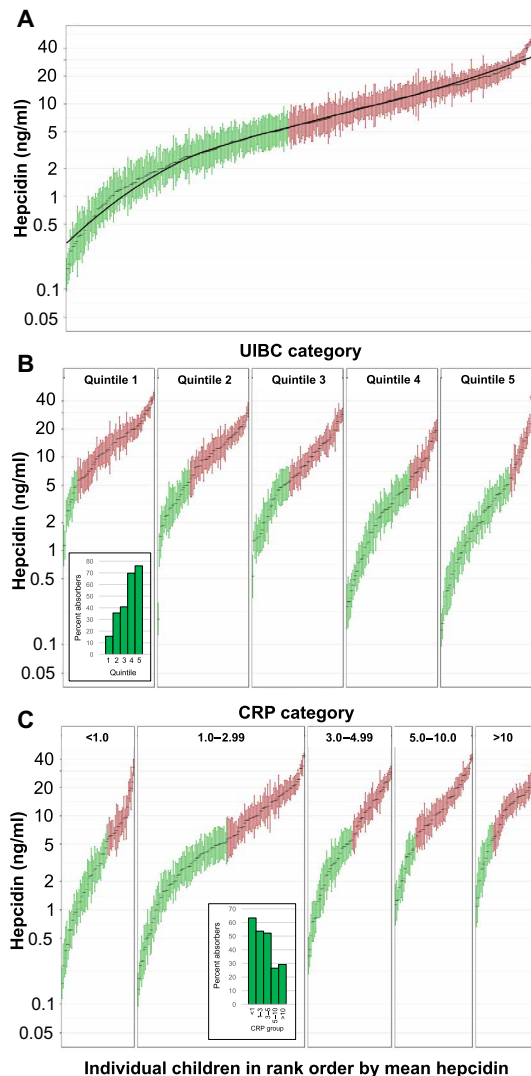
Fig. 1. Gambian children maintain highly characteristic hepcidin levels over 12 weeks of study.
