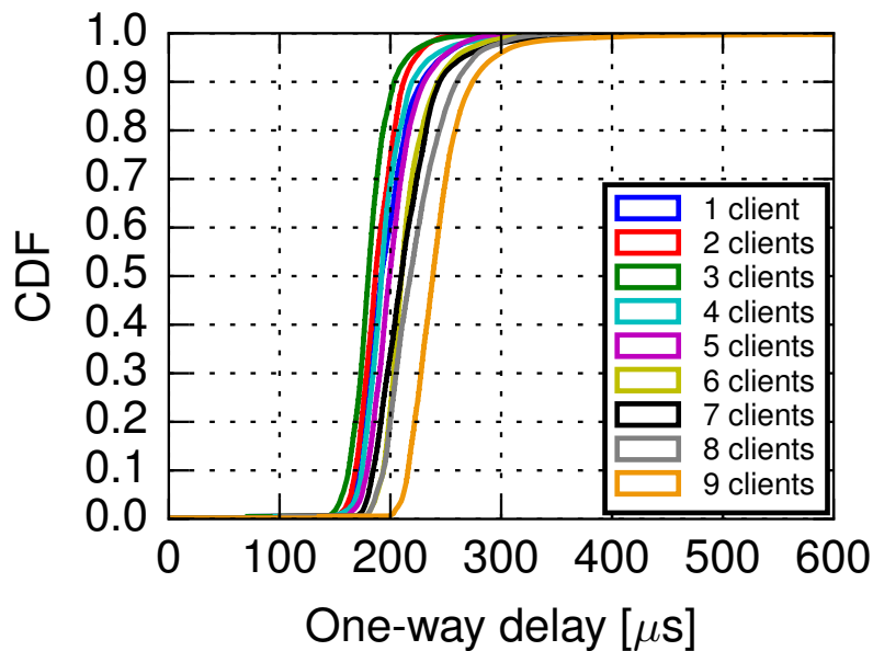
Figure 4.7: Varying the number of PTPd clients that synchronise with the PTPd master in EC2-USE.
