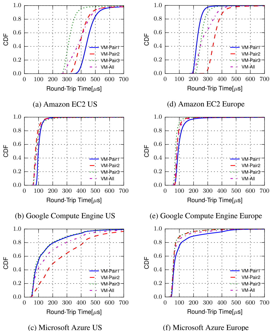
Figure 2.5: Measured RTTs within data centres for Amazon EC2, Google Compute Engine and Microsoft Azure in December 2016.
