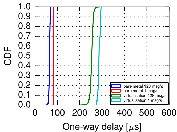
Figure 3.9: One-way delay reported by a PTPd client on a bare metal host and with virtualisation for different message frequencies.
