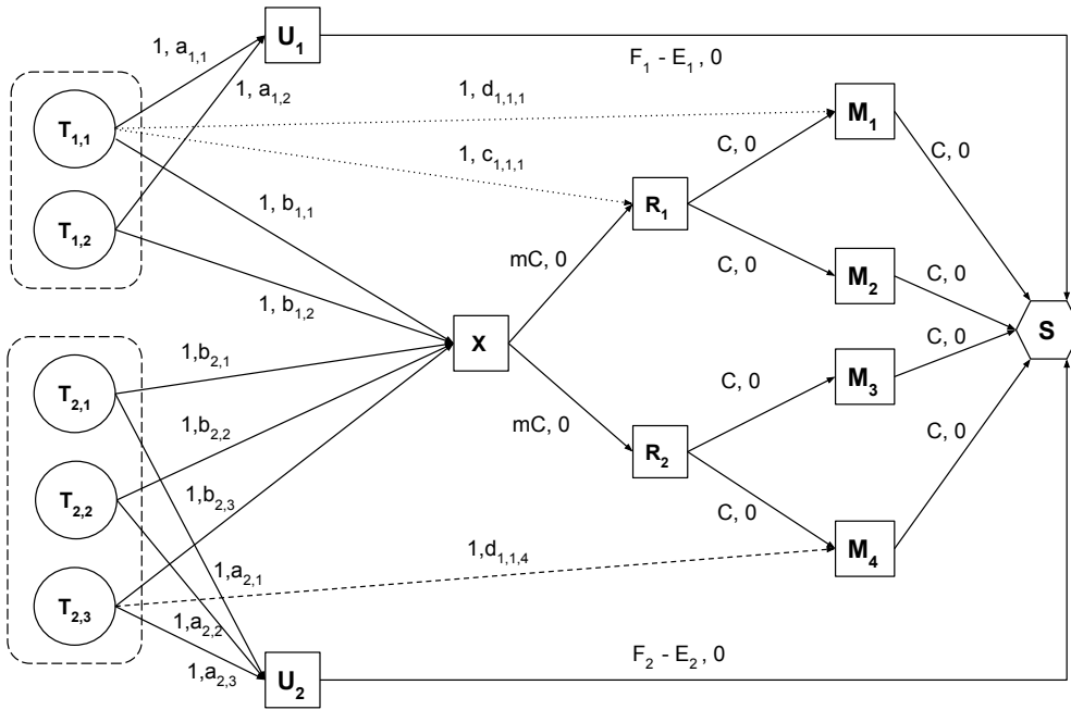
Figure 6.1: A general flow network with annotated capacities and costs on arcs. Job J_1 has tasks T_{1,1} and T_{1,2} . Job J_2 has tasks T_{2,1} , T_{2,2} and T_{2,3} . The unscheduled aggregator is U_1 . The machines in the cluster are M_1 , M_2 , M_3 and M_4 . Rack aggregators are R_1 and R_2 . The cluster aggregator is X . The sink vertex is S .
