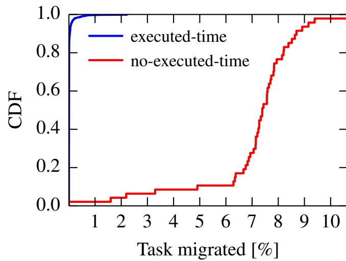
Figure 6.7: Percentage of migrated tasks for NoMora policy with preemption (parameters 105 and 110) on the Google workload.
