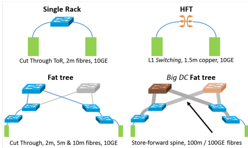
Figure 2.12: Different network topologies [ZGP + 17].
