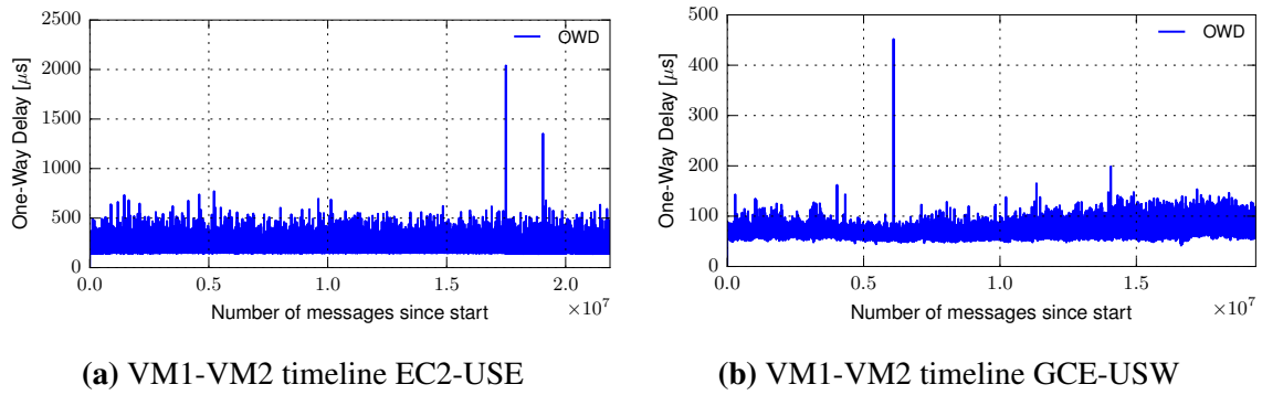
Figure 4.12: Measured OWD between VM1 and VM2 using the high message frequency.
