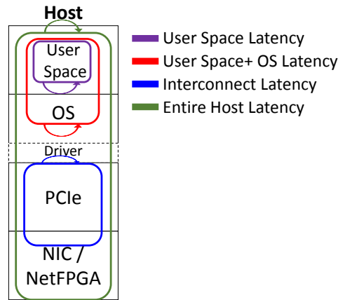
Figure 2.9: End-host tests setup [ZGP + 17].
