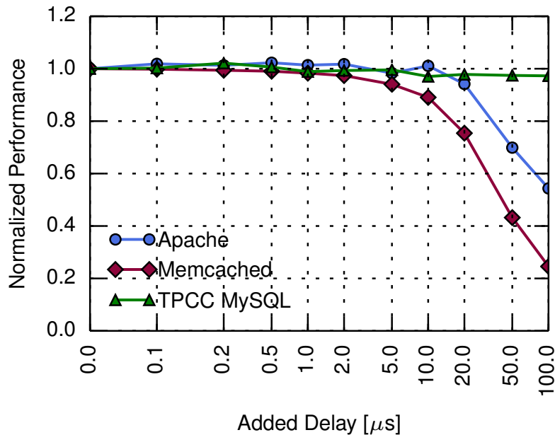
Figure 2.7: Network latency effect on application performance.
