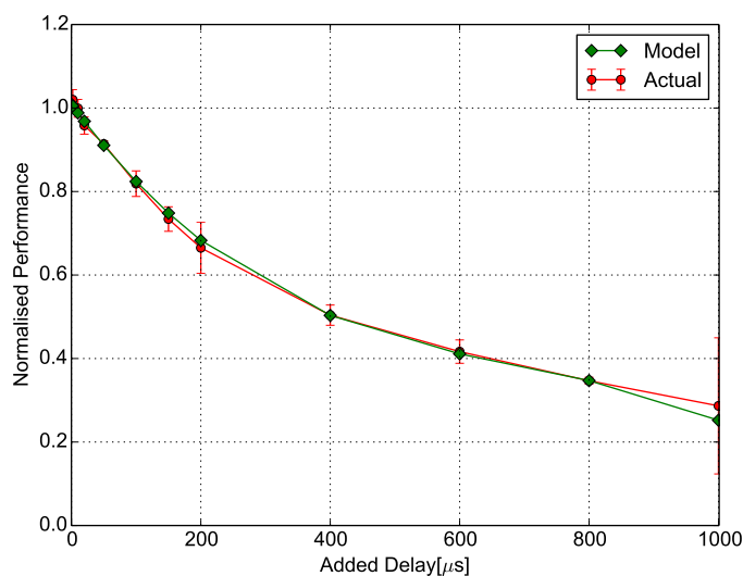
Figure 5.12: Polynomial function fitted to STRADS Lasso Regression experimental data.
