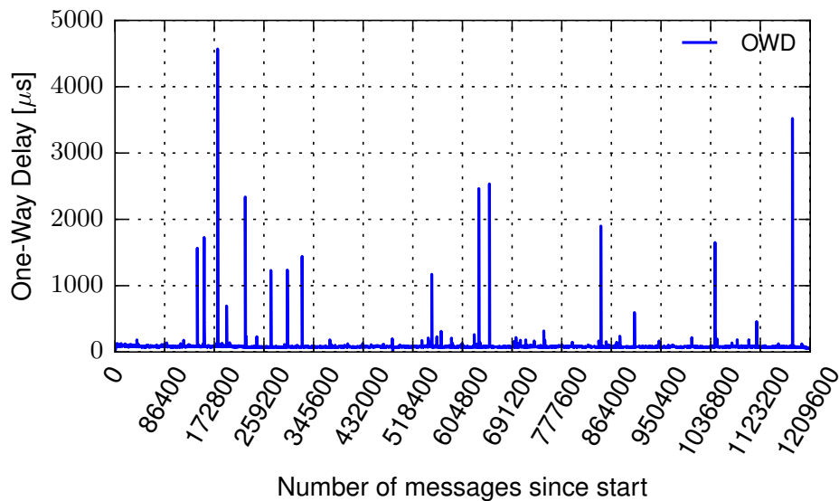
Figure 4.10: Measured OWD between VM1 and VM2 in GCE-USW data centre.
