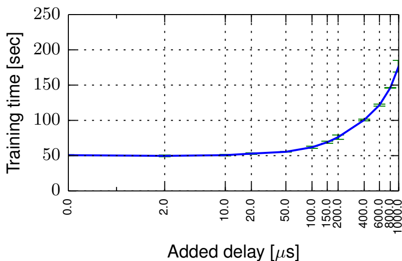
Figure 5.6: STRADS Lasso Regression training time for static latency injection.
