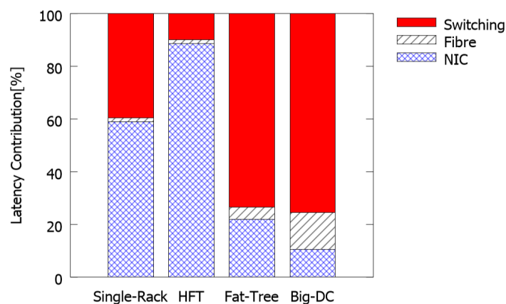
Figure 2.13: Network latency contributions [ZGP + 17].
