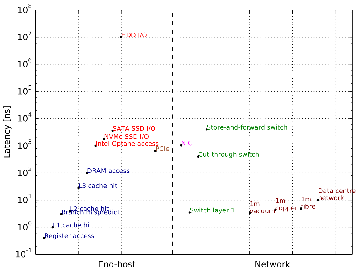
Figure 2.4: System events and their latencies.
