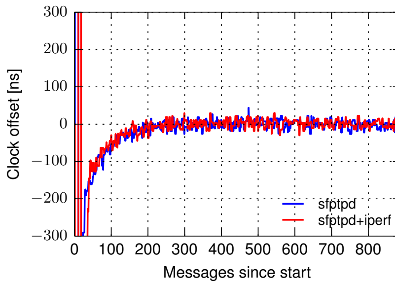
Figure 3.10: The clock offset reported by sfptpd is not affected by the iperf traffic, since it uses NIC hardware timestamping.
