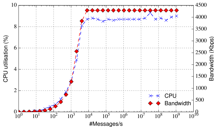
Figure 4.6: CPU and network bandwidth of the PTPd master running on a VM in the Azure-KS data centre synchronising with one PTPd client.
