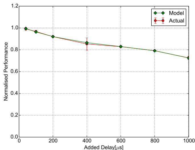
Figure 5.14: Polynomial function fitted to Tensorflow handwritten digit recognition experimental data.
