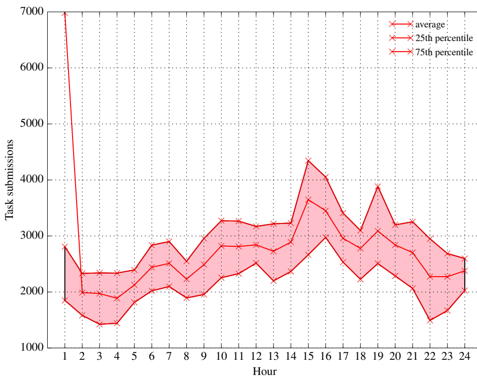
Figure 2.14: Azure workload number of task arrivals per hour - average, 25 th and 75 th percentiles.
