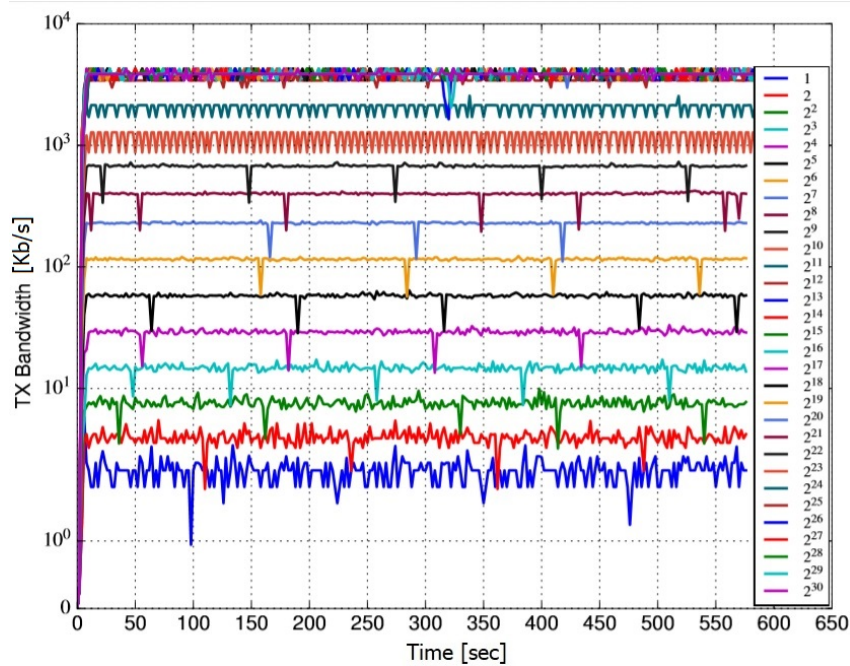
Figure 4.5: Send network bandwidth of the PTPd master running on a VM in the Azure-KS data centre synchronising with one PTPd client.
