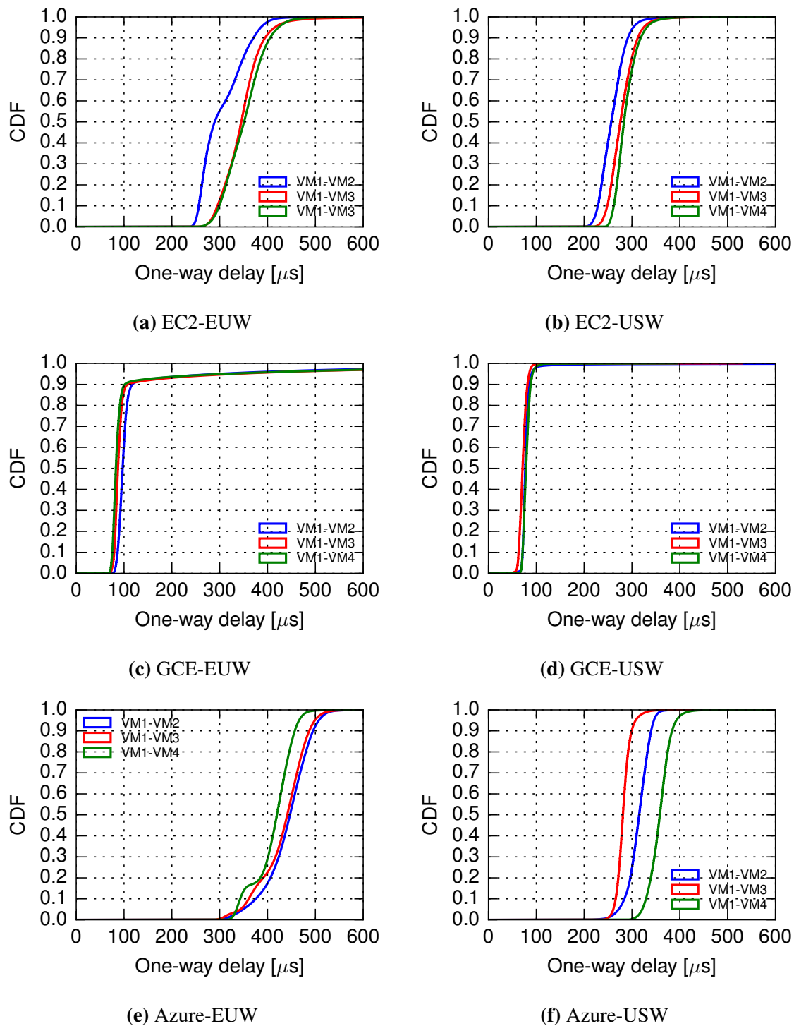
Figure 4.8: CDF of OWD in different data centres using the low message frequency.
