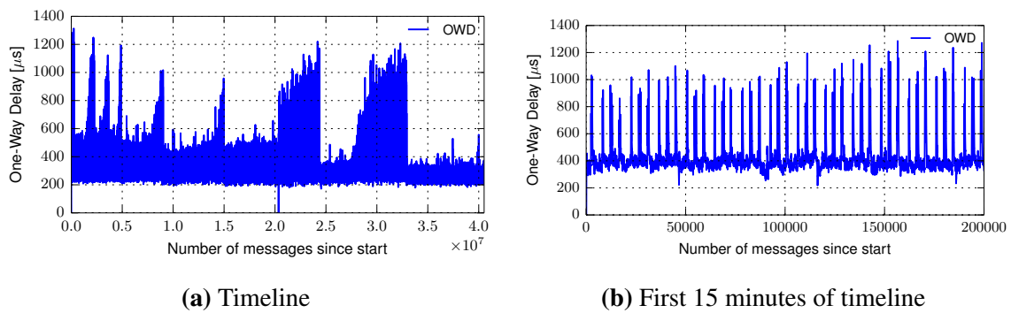
Figure 4.13: Measured OWD between VM1 and VM2 in Azure-UKS using the high message frequency.
