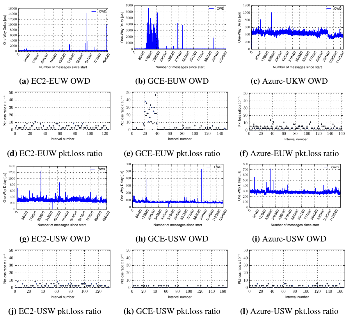
Figure 4.9: OWD and packet loss ratios over 1-hour intervals between VM1-VM3 in EU and US data centres over one week.
