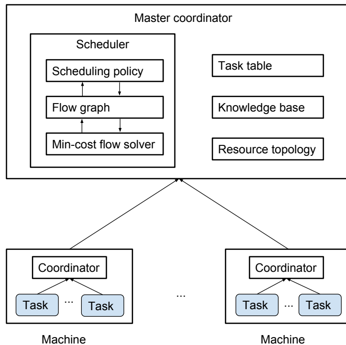
Figure 6.2: Firmament architecture.
