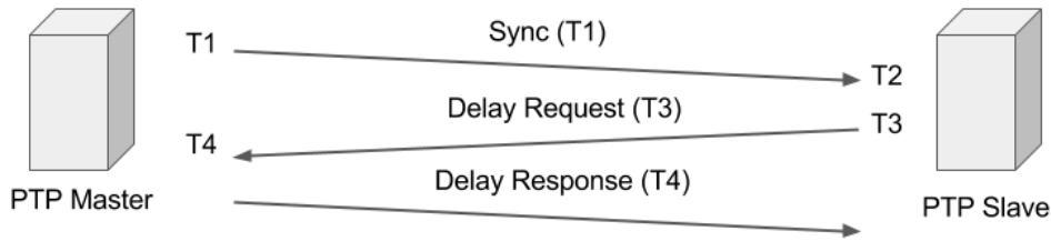
Figure 2.2: PTP protocol.
