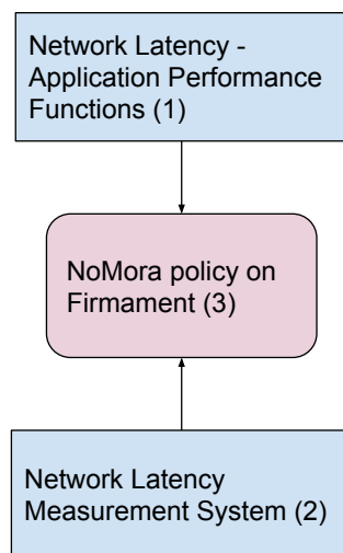
Figure 6.3: NoMora architecture.
