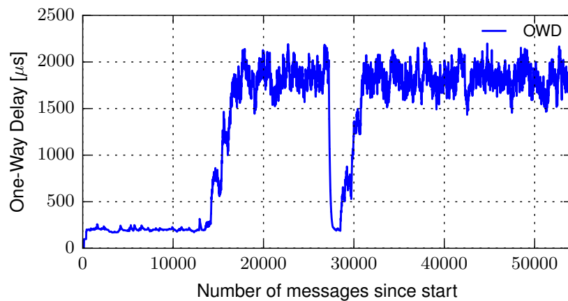
Figure 4.14: Measured OWD between VM1 and VM10 in EC2-USE data centre.
