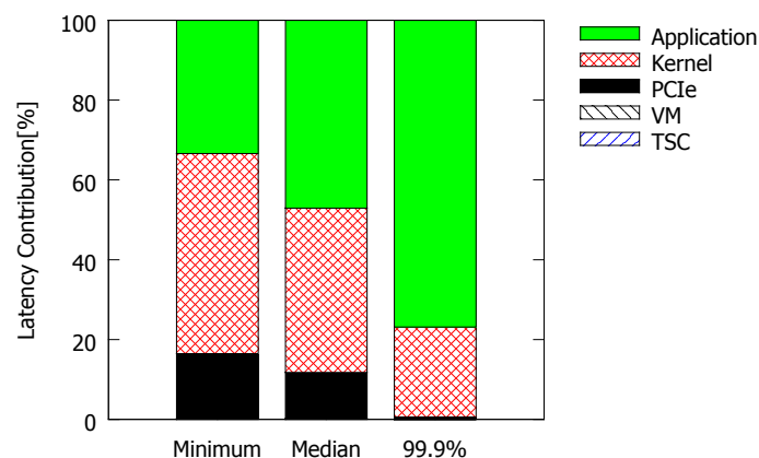
Figure 2.11: End-host latency contribution [ZGP + 17].
