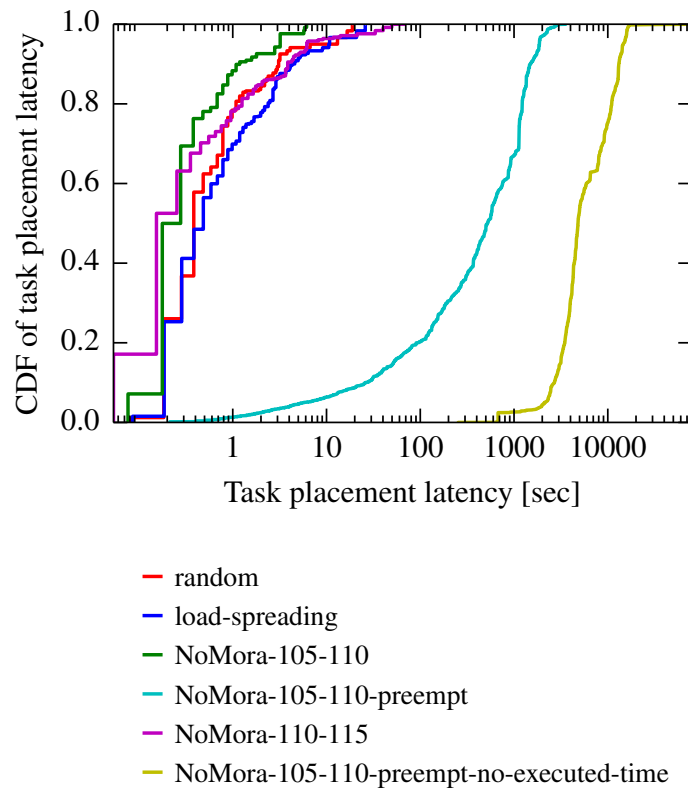
Figure 6.8: Task placement latency for different policies on the Google workload.
