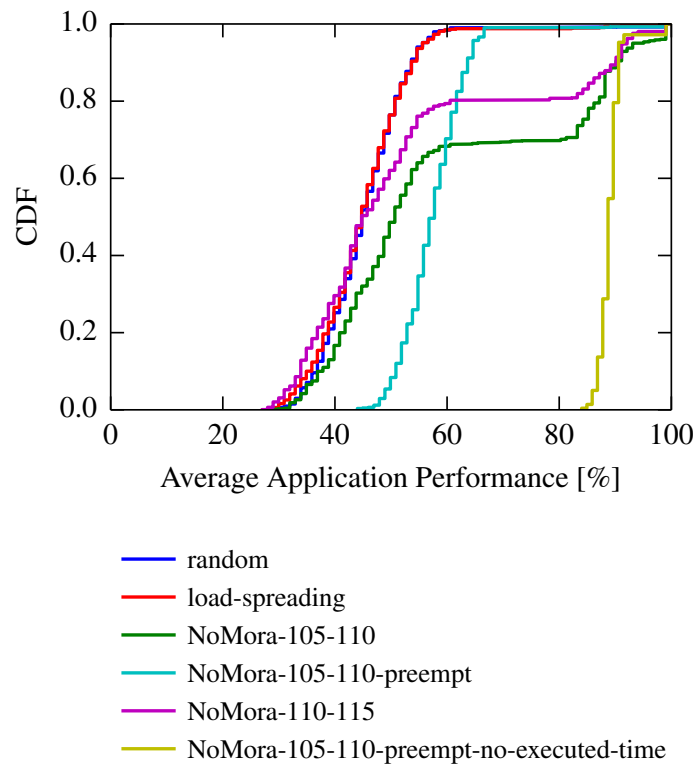
Figure 6.5: Average application performance for different policies on the Google workload.
