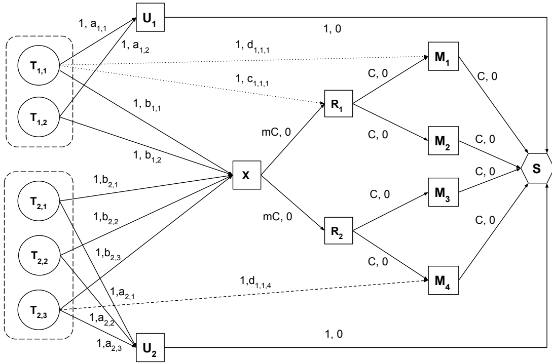
Figure 6.4: NoMora flow network with annotated capacities and costs on arcs.
