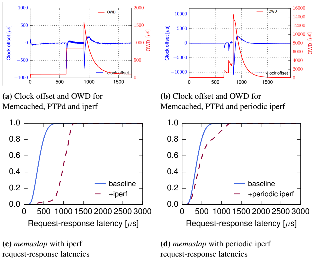
Figure 3.6: Network congestion effect on PTPd measurements and on memaslap 's performance.
