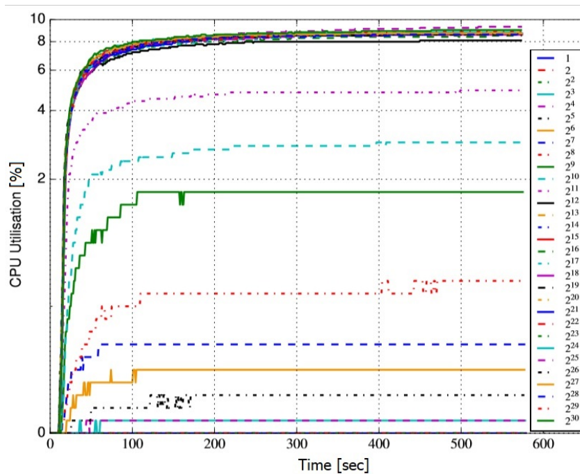
Figure 4.3: CPU utilisation of the PTPd master running on a VM in the Azure-KS data centre synchronising with one PTPd client.
