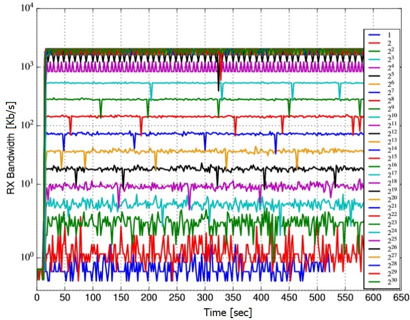
Figure 4.4: Receive network bandwidth of the PTPd master running on a VM in the Azure-KS data centre synchronising with one PTPd client.
