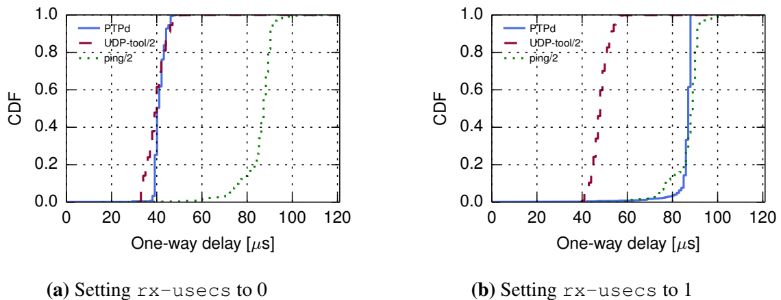
Figure 3.4: RTT/2 reported by ping and the UDP-based tool that uses the TSC [ZGP + 17], and one-way delay reported by PTPd
