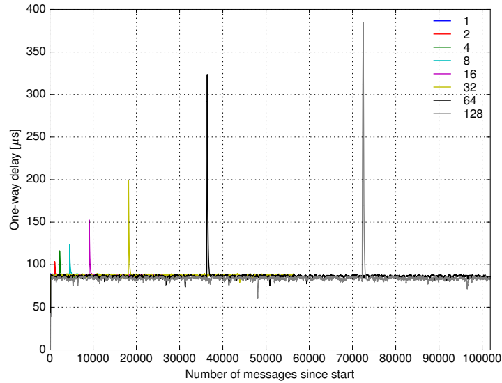
Figure 3.8: Number of messages needed for the one-way delay to return to normal values after network congestion caused by an iperf stream of 1s for different message frequencies.
