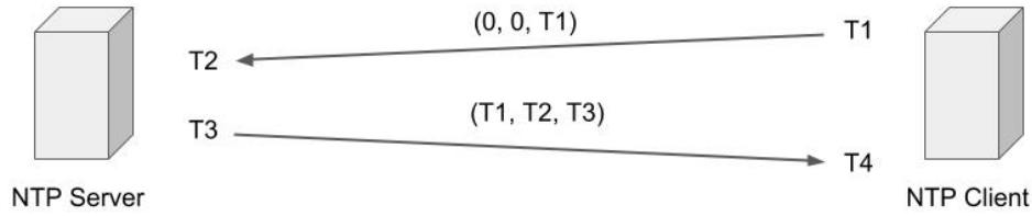
Figure 2.1: NTP protocol one-step mode.
