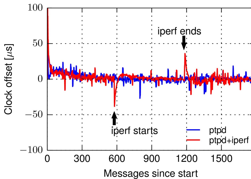
Figure 3.11: The clock offset reported by PTPd is adversely affected by the iperf traffic because of end-host interference.
