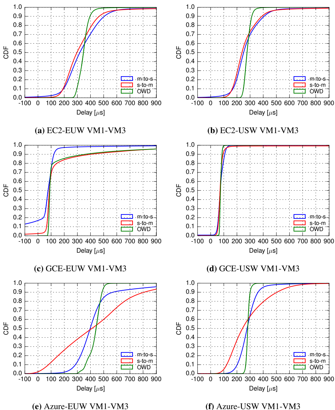
Figure 4.15: CDF for the master-to-slave (m-to-s) delay, slave-to-master (s-to-m) delay and OWD in different data centres.
