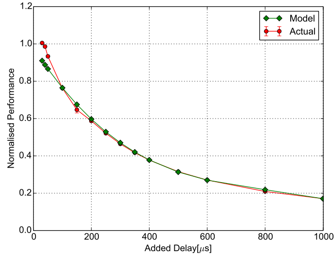
Figure 5.11: Polynomial function fitted to Memcached experimental data.
