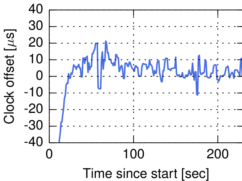
Figure 3.2: The slave's clock offset is within 20\mu\text{s} of the master's clock after less than five minutes after PTPd's start-up.
