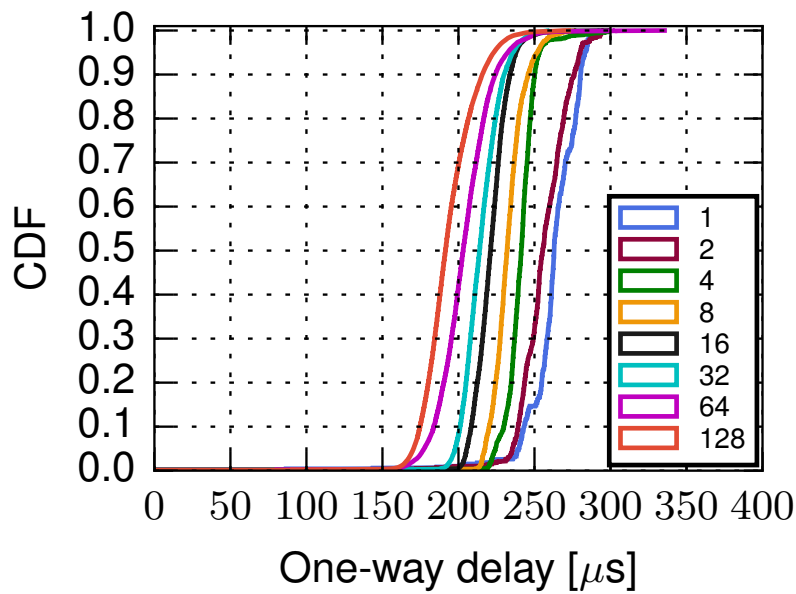
Figure 4.2: OWD measured using PTPd for periods of 15 minutes between two VMs in Azure-KS.
