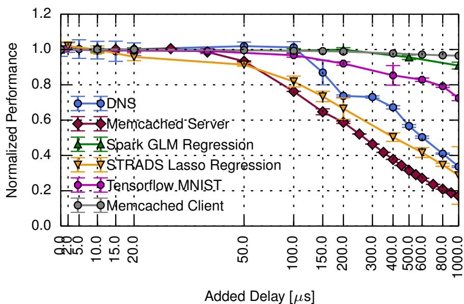
Figure 5.9: The effect of injected static latency on typical cloud applications' performance.
