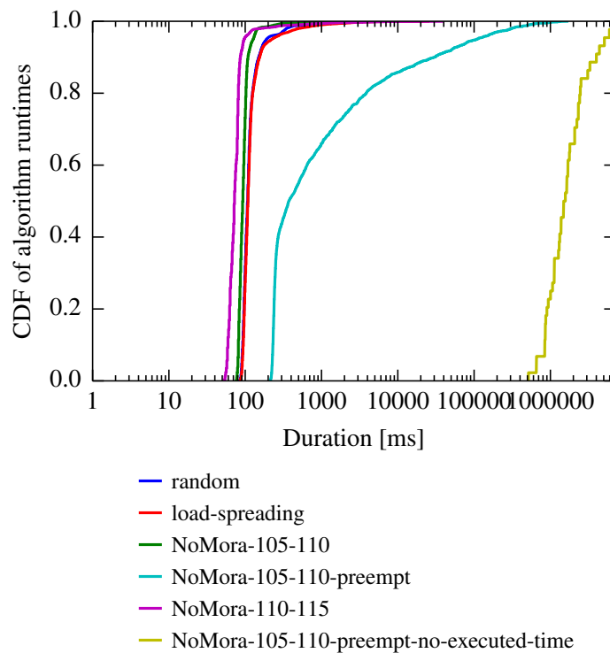
Figure 6.6: Algorithm runtime for different policies on the Google workload.
