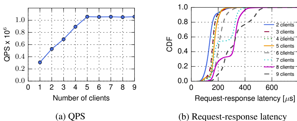
Figure 5.2: Baseline analysis to determine the maximum QPS that can be achieved by the Memcached server.
