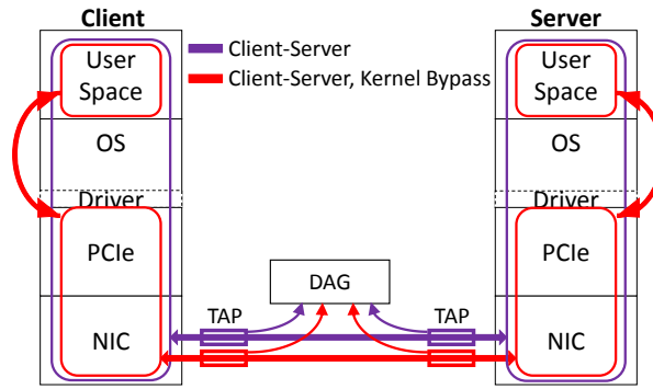
Figure 2.10: Client-server tests setup [ZGP + 17].
