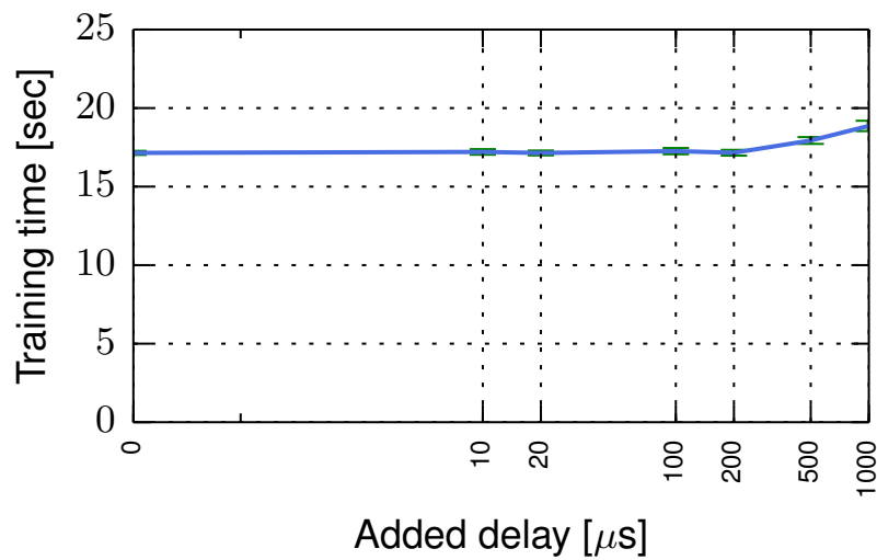
Figure 5.7: Spark GLM Regression training time for static latency injection.
