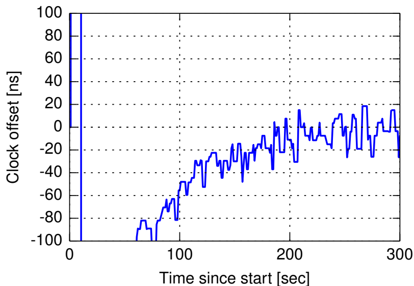
Figure 3.3: The slave's clock offset is within 40\text{ns} of the master's clock after less than five minutes after Solarflare's PTP daemon start-up.
