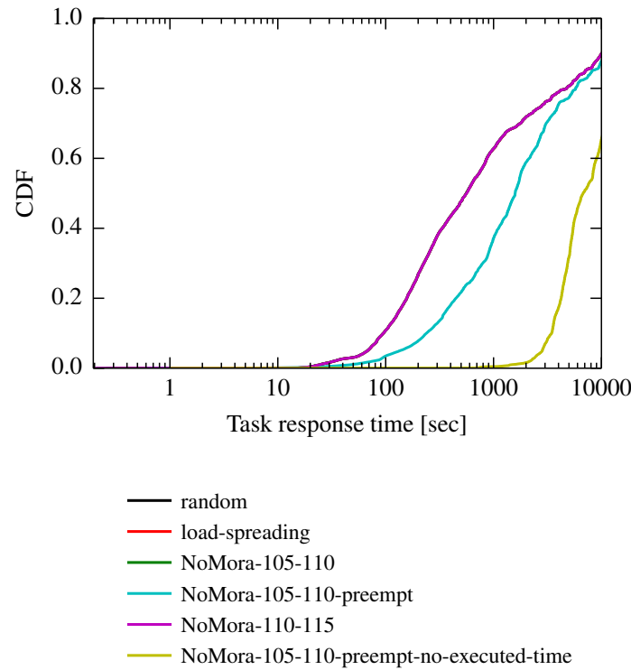
Figure 6.9: Task response time for different policies on the Google workload.
