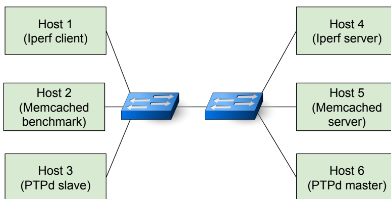
Figure 3.1: Testbed to analyse PTPd’s behaviour under different network conditions.
