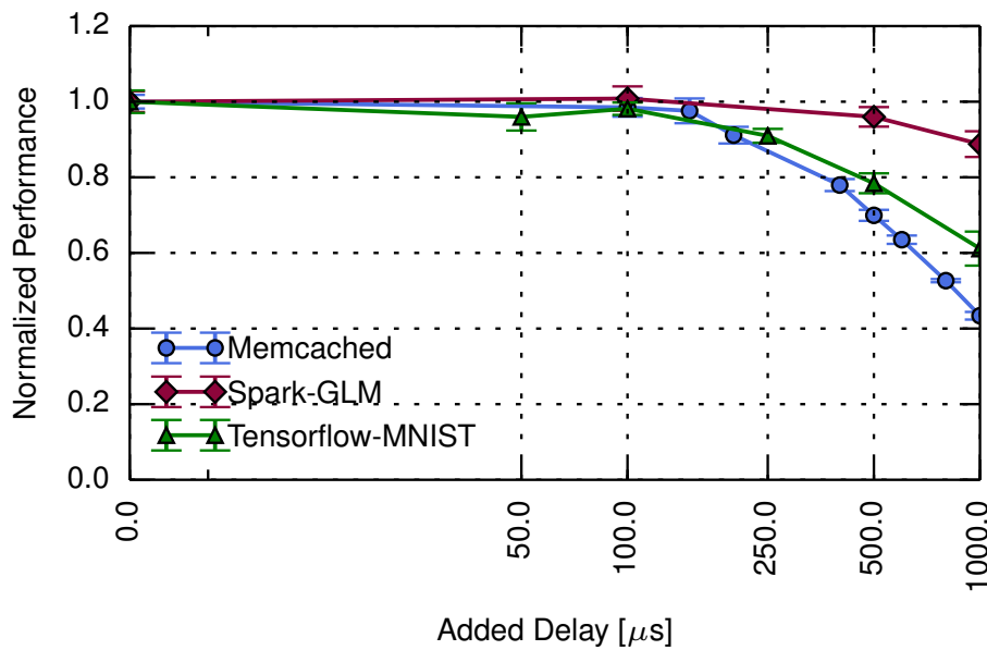
Figure 5.10: The effect of injected static latency on typical cloud applications’ performance running on cloud hardware.
