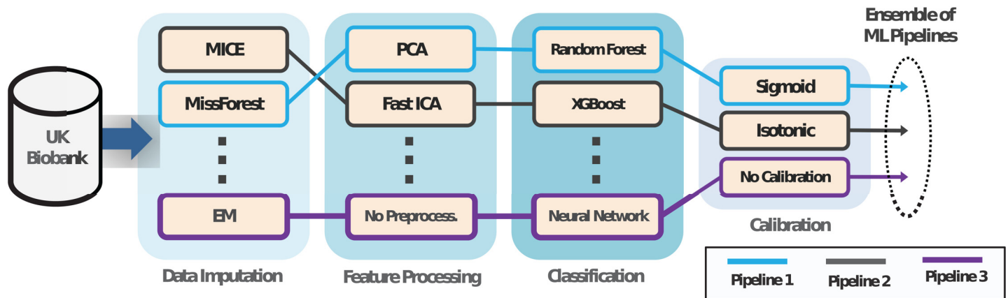
Fig 1. An illustrative schematic for AutoPrognosis. In this depiction, AutoPrognosis constructs an ensemble of three ML pipelines. Pipeline 1 uses the MissForest algorithm to impute missing data, and then compresses the data into a lower-dimensional space using the principal component analysis (PCA) algorithm, before using the random forest algorithm to issue predictions. Pipelines 2 and 3 use different algorithms for imputation, feature processing, classification and calibration. AutoPrognosis uses the algorithm in [19] to make decisions on what pipelines to select and how to tune the pipelines' parameters.
