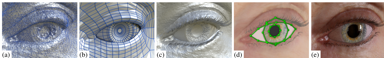
Figure 2: An overview of our model preparation process: Dense 3D head scans (1.4 million polygons) (a) are first retopologised into an optimal form for animation (9,005 polygons) (b). High resolution skin surface details are restored by displacement maps (c), and 3D iris and eyelid landmarks are annotated manually (d). A sample rendering is shown (e).
