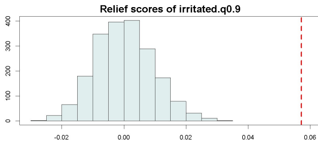
FIGURE 1. THE DASHED LINE CORRESPONDING TO OBSERVED RELIEF SCORE=0.057 FOR IRRITATED.Q0.9 VARIABLE IS SUFFICIENTLY FAR AWAY FROM THE CENTRE OF NORMAL DISTRIBUTION OF THE VARIABLE'S RELIEF SCORES BASED ON 2000 PERMUTATIONS OF LABELS. THIS INDICATES PREDICTIVE POWER FOR IRRITATE.Q0.9.
