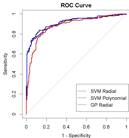
FIGURE 3. ROC CURVES OF THE 3 TOP MODELS
