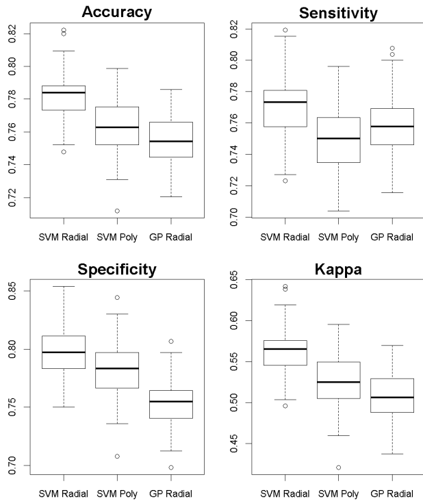
FIGURE 2. BOXPLOTS SHOWING PERFORMANCE RESULTS OF THE TOP 3 MODELS IN MONTE CARLO 100 EXPERIMENTS
