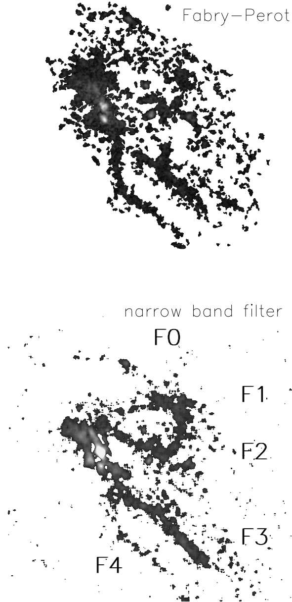
Fig. 3. Upper panel: H\alpha Fabry-Perot image (Chemin et al. 2005). Lower panel: H\alpha + [NII] narrow band image from Goldmine (Gavazzi et al. 2003) where a median filter of 7 pixels has been applied. The filaments F0–F4 mentioned in the text are labelled as F0–F4. Note that the greyscales are inverted (bright colors correspond to high surface brightness) to enhance the visibility of low surface brightness emission.
