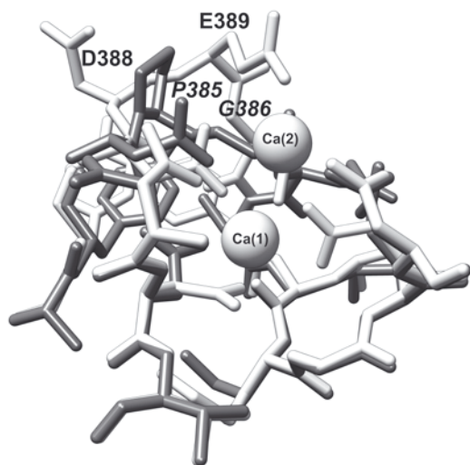
Figure 4. Superposition of residues from the area of calcium ion binding.
