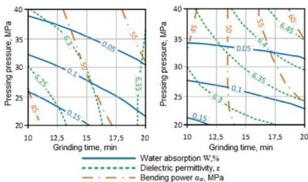
Fig. 4 Dependence of water absorption, dielectric permittivity and tensile strength in bending of samples of the composition “2” scorched at temperatures 1,300 and 1,350 °C from technological parameters
