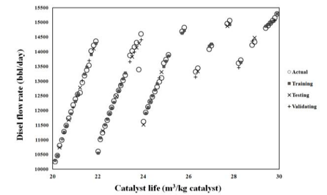
Figure 7 A comparison between simulated values with actual data for the diesel yield
