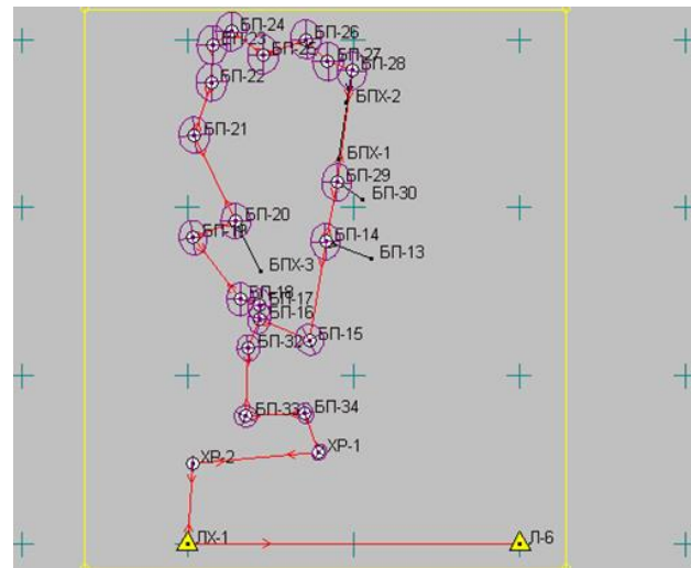
Fig. 2. Scheme of the underground geodetic network
