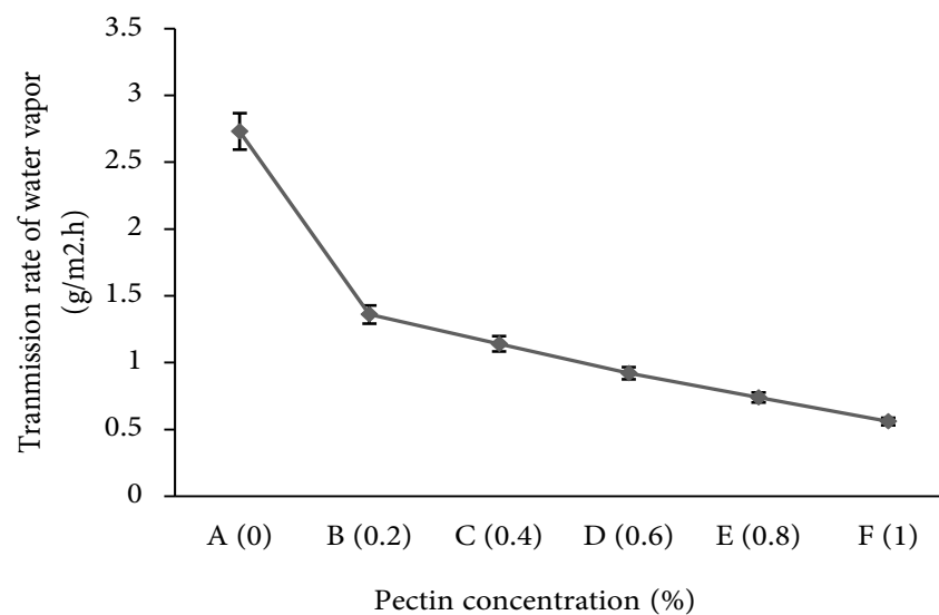
Figure 5 The transmission of water vapor of edible film from gelatin red snapper ( Lutjanus argentimaculatus ) by the addition of pectin.
