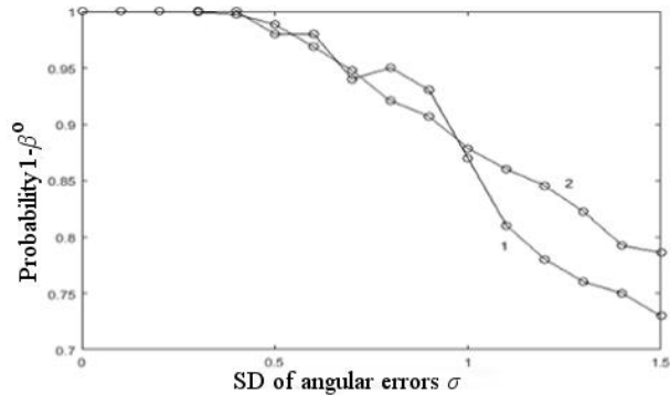
Figure 7. Estimated probability 1-\beta^\circ of spurious solution for early diagnostics of geomagnetic storms versus SD of angular errors \sigma
