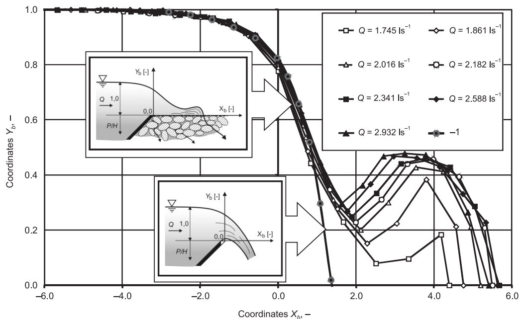
Fig. 3. Dimensionless curves of the free water surface on the permeable sill (own research): Q – according to own research, 1 – according to Khan & Steffler (1996) for sharp-crested weir
