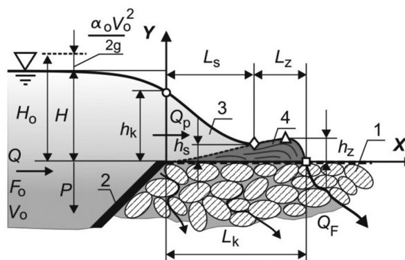
Fig. 1. Overflow stream of permeable sill: 1 – stone permeable sill, 2 – sharp-crested weir on upstream slope, 3 – free flow zone, 4 – wave intake (inlet) zone
