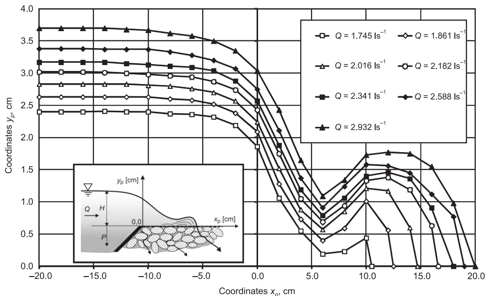
Fig. 2. Dimensional curves of the free water surface on the permeable sill
