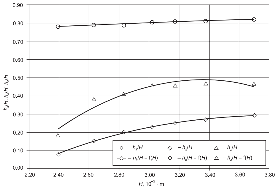
Fig. 4 . Dimensionless water depths on permeable sill
