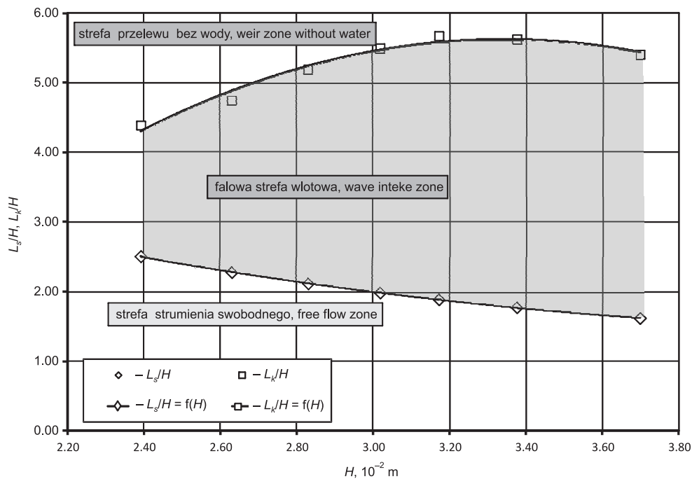
Fig. 5. Ranges of stream zones on the permeable sill
