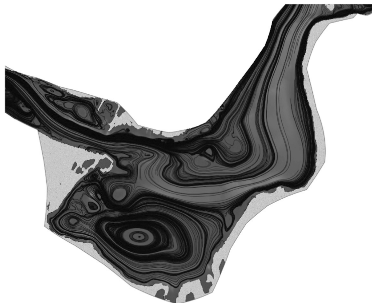
Fig. 7. Flow lines at Dębe reservoir on January 5, 2017 calculated by CCHE2D model with the influence of wind NW 5 \text{ m} \cdot \text{s}^{-1}
