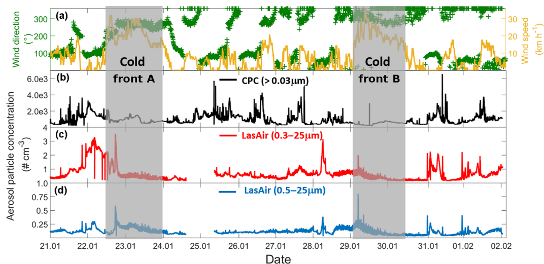
Figure 2. Time evolution of wind and aerosol particle concentration time series for the entire campaign (21 January–2 February 2017). (a) Time series of the wind speed (yellow) and wind direction (green), (b) particle concentration measured by the CPC, (c) particle concentration measured by the LasAir full-size range (0.3 to 25 \mu\text{m} ), and (d) particle concentration measured by the LasAir for particles > 500 nm (0.5 to 25 \mu\text{m} ). Grey areas denote the periods affected by cold fronts A and B. Each tick mark on the x axis corresponds to midnight local time.
