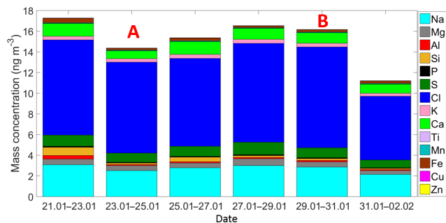
Figure 3. Time series of the ambient aerosol mass concentration and bulk chemical composition as measured by the XRF. Each sample was collected for 48 h starting at 12:00 h local time. A and B indicate that those samples were partially influenced by the passage of the cold front A and the cold front B, respectively.
