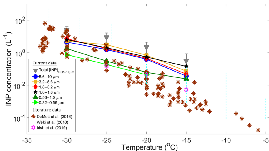
Figure 4. Summary of average INP concentrations as a function of temperature and particle size (solid symbols). Total [INP] are represented by the grey triangles, whereas the brown asterisks, light blue dotted lines, and purple stars are data from DeMott et al. (2016), Welti et al. (2018), and Irish et al. (2019), respectively. The upper and lower detection limits of the MOUDI-DFT are 30 and 0.01 \text{ L}^{-1} .
