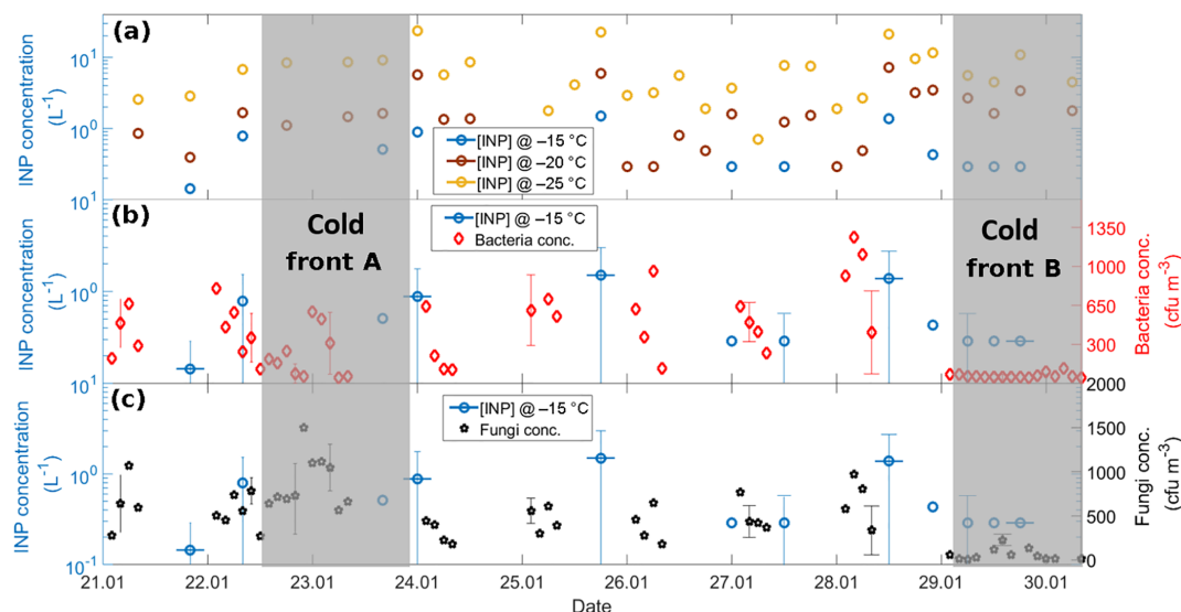
Figure 9. (a) Time series of the [INP] at -15 (blue), -20 (brown), and -25 °C (yellow), (b) time series of the [INP] at -15 °C (blue) together with bacteria concentration (red), and (c) time series of the [INP] at -15 °C (blue) together with fungal concentration (black). Each x -axis tick corresponds to 06:00 local time. The horizontal uncertainty bars indicate the time span of the MOUDI-DFT measurements, i.e., 6 h. Grey areas denote the periods affected by cold fronts A and B.
