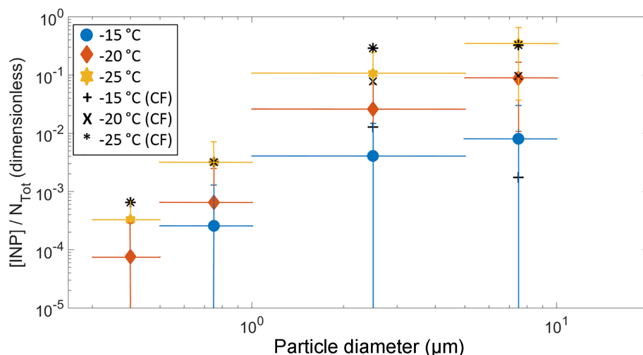
Figure 7. The fraction of aerosol particles acting as an INP ( [INP]/N_{Tot} ) as a function of particle size at -15 , -20 , and -25\text{ }^\circ\text{C} . N_{Tot} refers to the number of aerosol particles in a given size range measured by the LasAir. The solid colored symbols represent the entire campaign, while the black symbols represent the samples collected under the influence of the cold fronts.
