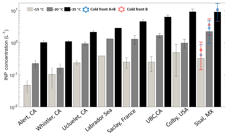
Figure 5. Mean INP number concentrations at droplet freezing temperatures of -15 (light gray), -20 (dark gray), and -25 °C (black). The blue and red stars represent the mean INP concentration during the cold fronts A and B and cold front B, respectively. Uncertainties are given as the standard uncertainty of the mean (adapted from Mason et al., 2016).
