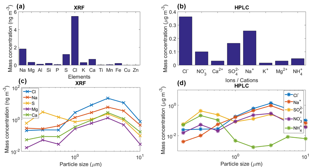
Figure 8. (a) Mean mass concentration of 14 detected elements for the collected aerosol particles using XRF, (b) mean mass concentration of eight detected ions for the collected aerosol particles using HPLC, (c) and (d) mean mass size distribution of the main five detected elements/ions with the XRF and HPLC. These results are the average for the whole sampling period.
