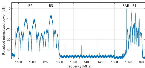
Figure 5 Power Spectra of Beidou 3 M13 captured October 1, 2018.
