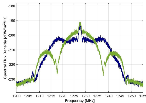
Figure 4 L2 spectral flux density of the GPS Block IIR-M satellite G055 (NAVSTAR 60). Blue: nominal transmission including M-code on May 11, 2018 at 05:07 UTC. Green: flex power mode without M-code transmission on April 17, 2018 at 09:02 UTC.
