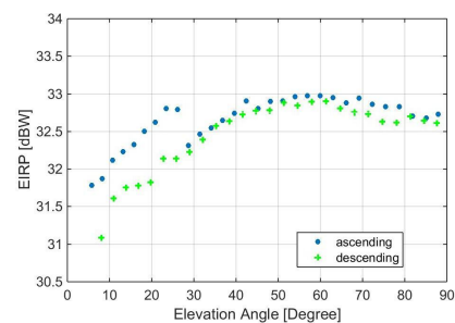
Figure 2 L1 Equivalent Isotropically Radiated Power (EIRP) of G065. 23 March 2018: nominal transmission including C/A-, P(Y)-, and M-code until approximately 27 degree elevation, then switch to flex power mode resulting in an EIRP reduction of about 0.6 dB
