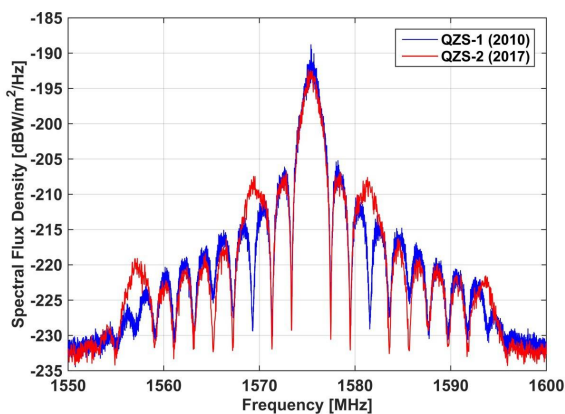
Figure 8 QZS-1 and QZS-2 L1 spectral flux density [Thoelert 2017].
