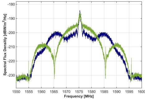
Figure 3 L1 spectral flux density of the GPS Block IIR-M satellite G055 (NAVSTAR 60). Blue: nominal transmission including M-code on May 11, 2018 at 05:06 UTC. Green: flex power mode without M-code transmission on April 17, 2018 at 09:01 UTC
