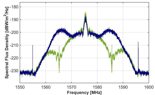
Figure 1 L1 spectral flux density of the GPS Block IIF satellite G065 (NAVSTAR 67) on 25 March 2018. Blue: nominal transmission including M-code at 10:34 UTC. Green: flex power mode without M-code transmission at 10:42 UTC
