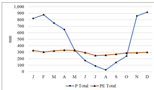
Fig. 3. Monthly precipitation P and potential evapotranspiration PE .
