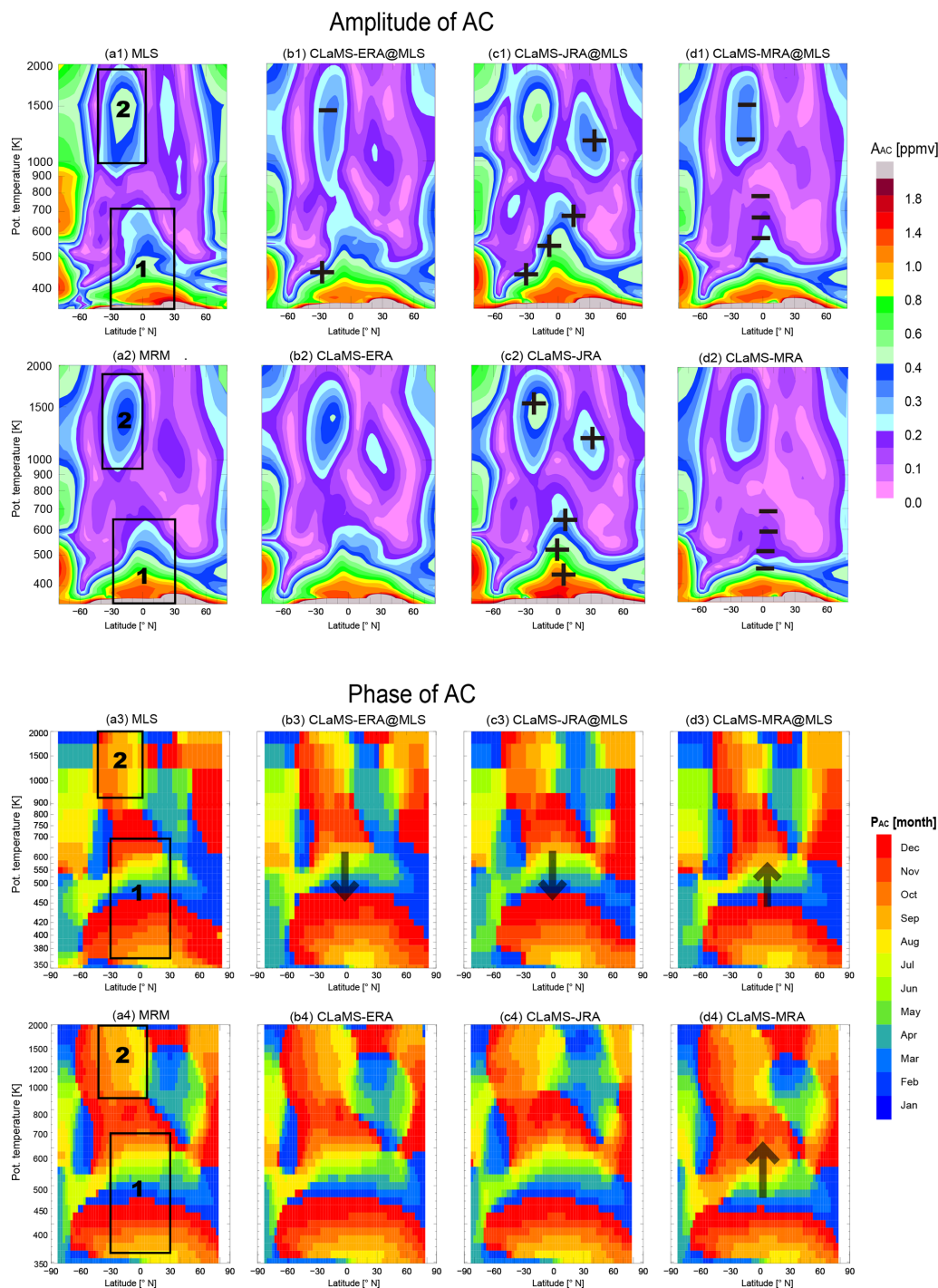
Figure 7. AC amplitudes ( A_{AC} ) and corresponding phases ( P_{AC} ) during the MLS period ( \sim 2005 – 2013 , the first and third rows) and the entire CLaMS period (1980– 2013 , the second and fourth rows). The leftmost panels show A_{AC} and P_{AC} based on Aura MLS observations (a1, a3) and the mean of the three reanalysis-driven models (MRM, a2, a4). The corresponding A_{AC} values from CLaMS-ERA, CLaMS-JRA and CLaMS-MRA are shown in the rightmost three panels of each row. Overlaid “+” and “-” symbols in panels (b1)–(d1) and (b2)–(d2) demonstrate major differences by more than \pm 30\% in simulated A_{AC} relative to the benchmark estimate shown in the corresponding leftmost panel. Arrows in panels (b3)–(d3) and (b4)–(d4) indicate the major region with phase differences by more than 1 month against the benchmark estimate of P_{AC} shown in the corresponding leftmost panel. The upward arrows show phase lagging behind of the benchmark phase while the downward arrows show phase ahead of the benchmark phase.
