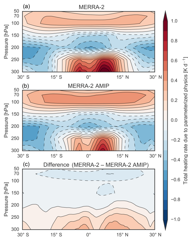
Figure D1. Comparison of time-mean zonal-mean diabatic heating rates in the tropical ( 30^{\circ}\text{N} – 30^{\circ}\text{S} ) lower stratosphere between the MERRA-2 reanalysis (a) and the MERRA-2 AMIP ensemble mean (b) over 1980–2017. Differences between MERRA-2 and MERRA-2 AMIP are shown in (c).
