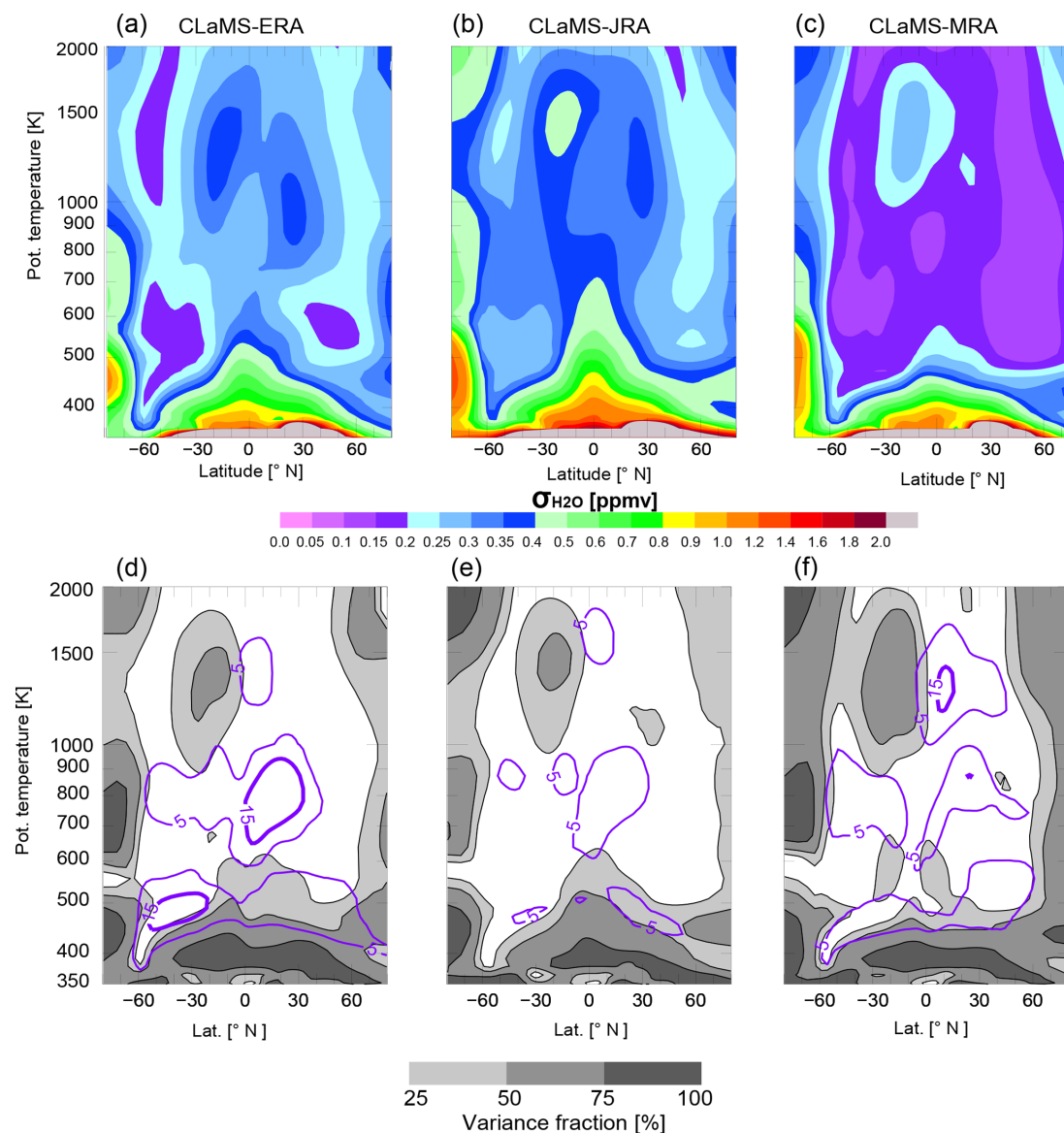
Figure 10. The standard deviation in monthly-mean H 2 O ( \sigma_{\text{H}_2\text{O}} ; upper row) and the fraction of AC and QBO variance relative to total variance (in %; d, e, f) for CLaMS-ERA (a, d), CLaMS-JRA (b, e) and CLaMS-MRA (c, f). Shading in the lower panels shows the variance fraction attributed to the annual cycle ( \sigma_{\text{H}_2\text{O}}^2 / \sigma_{\text{H}_2\text{O}}^2 ), while purple contours show the variance fraction attributed to the QBO ( \sigma_{\text{H}_2\text{O}}^2 / \sigma_{\text{H}_2\text{O}}^2 ).
