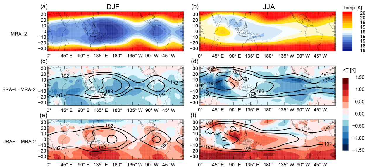
Figure 5. Climatological mean cold point tropopause temperatures during boreal winter (DJF, a, c, e) and boreal summer (JJA, b, d, f) from MERRA-2 (a, b), along with differences in ERA-I (c, d) and JRA-55 (e, f) relative to MERRA-2. Isolines in the middle and lower rows show absolute values of tropopause temperature. Cold point tropopause temperatures are defined here as minimum temperatures between \theta = 360 K and \theta = 420 K.
