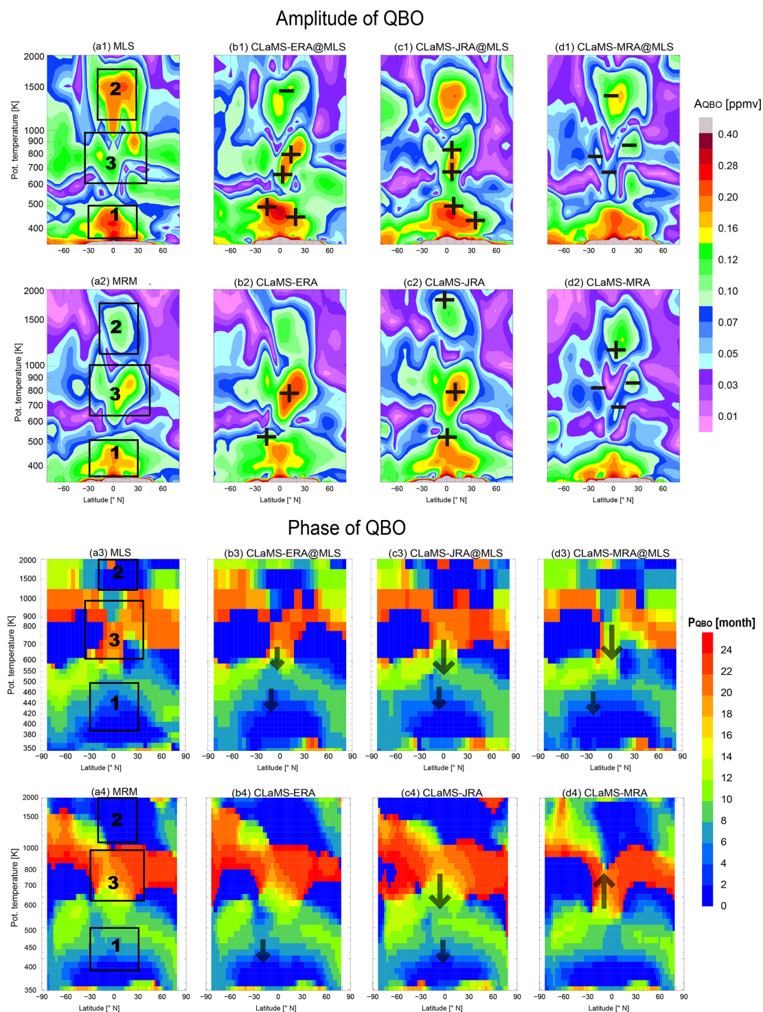
Figure 8. Same as Fig.7 but for QBO amplitudes and phases. Note that the scale of color bars are different from that in Fig. 7. Overlaid “+” and “-” symbols in panels (b1)–(d1) and (b2)–(d2) demonstrate major differences by more than \pm 30\% in simulated QBO amplitudes relative to the benchmark estimate shown in the corresponding leftmost panel. The large and small arrows show the major region with phase differences by more than 1 and 3 months, respectively, against the benchmark P_{QBO} shown in the corresponding leftmost panel. The upward arrows show phase lagging behind of the benchmark phase while the downward arrows show phase ahead of the benchmark phase.
