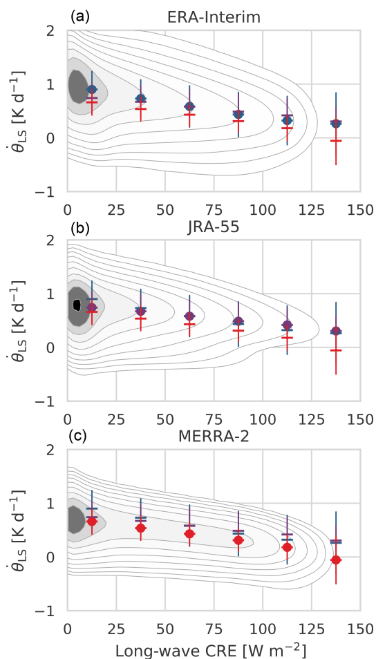
Figure 11. Joint distributions of daily-mean gridded diabatic heating rates ( \dot{\theta} ) in the tropical lower stratosphere ( \theta = 380 \text{ K} to \theta = 460 \text{ K} ) against the corresponding long-wave cloud radiative effect (LWCRE) based on ERA-I (a), JRA-55 (b) and MERRA-2 (c) during 1980–2013. The LWCRE is calculated as clear-sky minus all-sky outgoing long-wave radiation. Also shown are means and standard deviations of \dot{\theta}_{LS} composited into LWCRE bins in intervals of 25 \text{ W m}^{-2} starting from zero. Estimates based on ERA-I (blue), JRA-55 (purple) and MERRA-2 (red) are shown on all three panels to facilitate comparison. Distributions are based on variables archived on 1^\circ \times 1^\circ (ERA-I) and 1.25^\circ \times 1.25^\circ (JRA-55 and MERRA-2) latitude–longitude grids between 30^\circ \text{ S} and 30^\circ \text{ N} .
