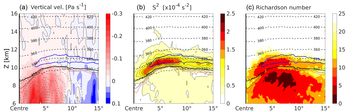
Figure 10. Vertical tropopause-based averaged cross section as in Fig. 9, but only north of the cyclone centre. (a) Filled contours show mean vertical velocity, solid thin black line the \omega = 0 \text{ Pa s}^{-1} isoline. Grey dashed lines are isolines of the cloud ice water content, steps as in Fig. 9. (b) Filled contour and solid black contour lines show squared vertical shear of horizontal wind S^2 . (c) Modified Richardson number mean Ri , with an inverted colour scale (red represents low values) to highlight the tendency toward turbulent motion. Blue solid bold line in all three panels shows the N_{\text{mean}}^2 = 6 \times 10^{-4} \text{ s}^{-2} isoline, dashed black lines the isentropes.
