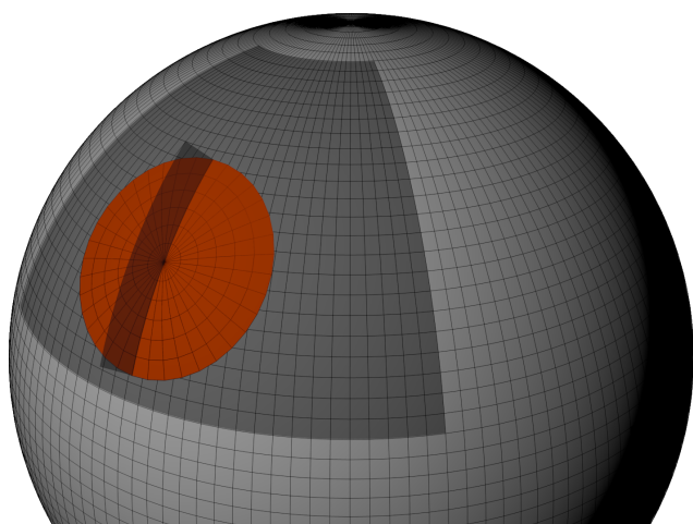
Figure 2. Schematic of the size of the analysed region (dark grey) in comparison to the full sphere, as well as the size of a rotated spheric polar coordinate system (orange) with \Theta_{\max} = 15^\circ radius. The dark grey semi-transparent upright plane illustrates (with exaggerated vertical extent) the vertical cross section aligned from north to south as displayed in Fig. 9.
