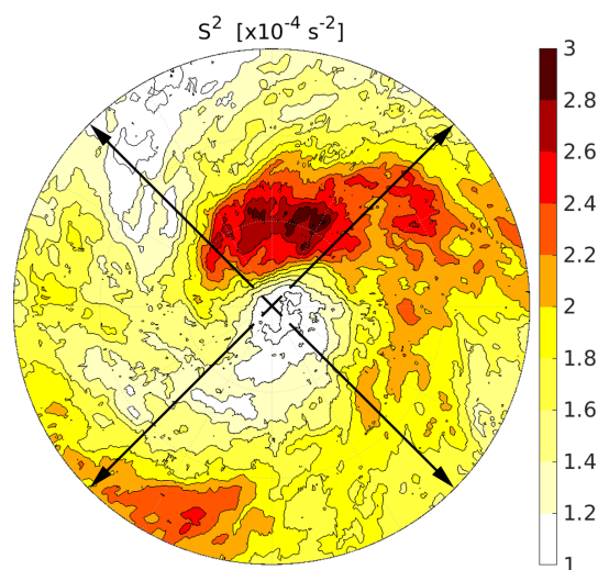
Figure 11. Composite of the vertical wind shear for the 76 strong cyclones with p_{\text{msl, min}} \leq 990 \text{ hPa} at the point in time of maximum intensity, averaged over the individual quasi-horizontal fields of maximum vertical wind shear S_{\text{max}}^2 found within 3 km above the lapse rate tropopause for each cyclone. The black arrows indicate the orientation of the vertical cross sections in Fig. 12.
