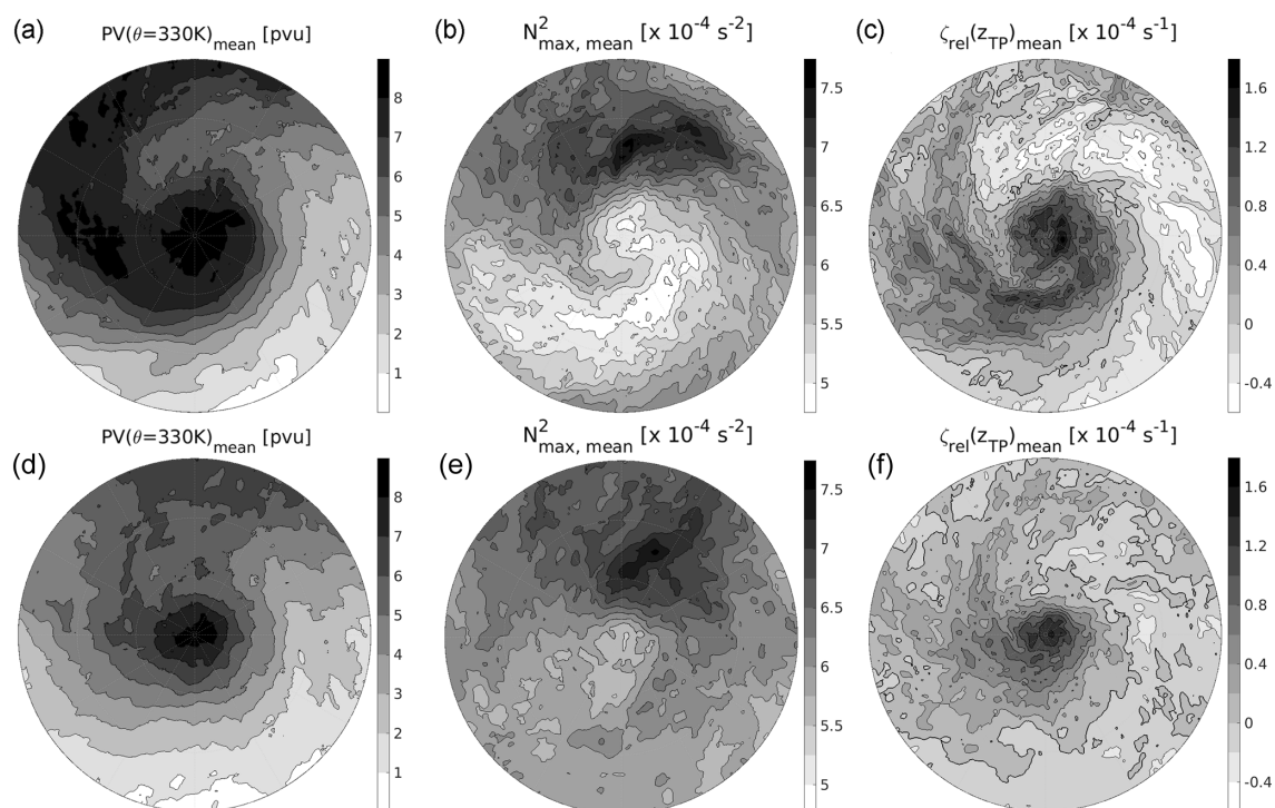
Figure 8. As in Fig. 7, but for (1) panels (a)–(c): for the 30 very strong cyclones with p_{\text{msl, min}} \leq 980 hPa, and (2) panels (d)–(f): the 54 weak cyclones with p_{\text{msl, min}} > 990 hPa.
