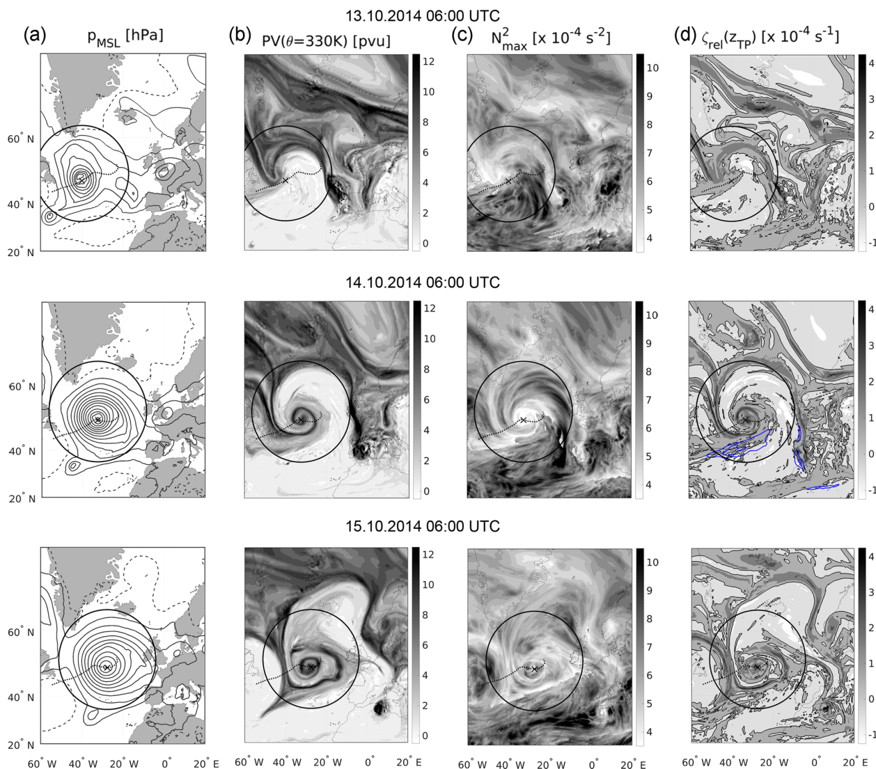
Figure 3. Evolution of a baroclinic wave-breaking event as seen in ECMWF IFS analysis data. The middle row represents 14 October 2014 at 06:00 UTC (the point in time of maximum cyclone intensity), and the upper and lower row show the situation 24 h prior and past the maximum intensity. Column (a) shows the pressure at mean sea level (solid lines p_{\text{msl}} \leq 1013 hPa, dashed lines p_{\text{msl}} > 1013 hPa, in steps of 5 hPa), (b) the IPV on 330 K, (c) the maximum of static stability N_{\text{max}}^2 within 3 km above the thermal tropopause as an indicator for the TIL strength, and (d) the relative vorticity at lapse rate tropopause height. Blue lines in the middle row show 40 and 50 m s -1 horizontal wind speed isolines at 200 hPa. The dashed black line shows the path of migration of the tracked cyclone, with the position of the cyclone centre at the point in time of the meteorological field displayed marked by the black \times . Black circles show the 15° radius used for the composites. Note the deformation of the circles due to the mercator projection.
