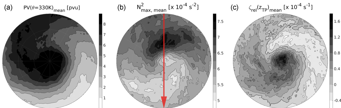
Figure 7. Composite of flow features for the 76 strong cyclones with p_{\text{msl, min}} \leq 990 hPa at the point in time of maximum intensity: (a) IPV on 330 K, (b) TIL strength N_{\text{max}}^2 , and (c) relative vorticity \zeta_{\text{rel}} at lapse rate tropopause height. The \zeta_{\text{rel}} = 0 \text{ s}^{-1} isoline is indicated by the black solid line. The red arrow in the middle indicates the orientation of the cross section in Fig. 9.
