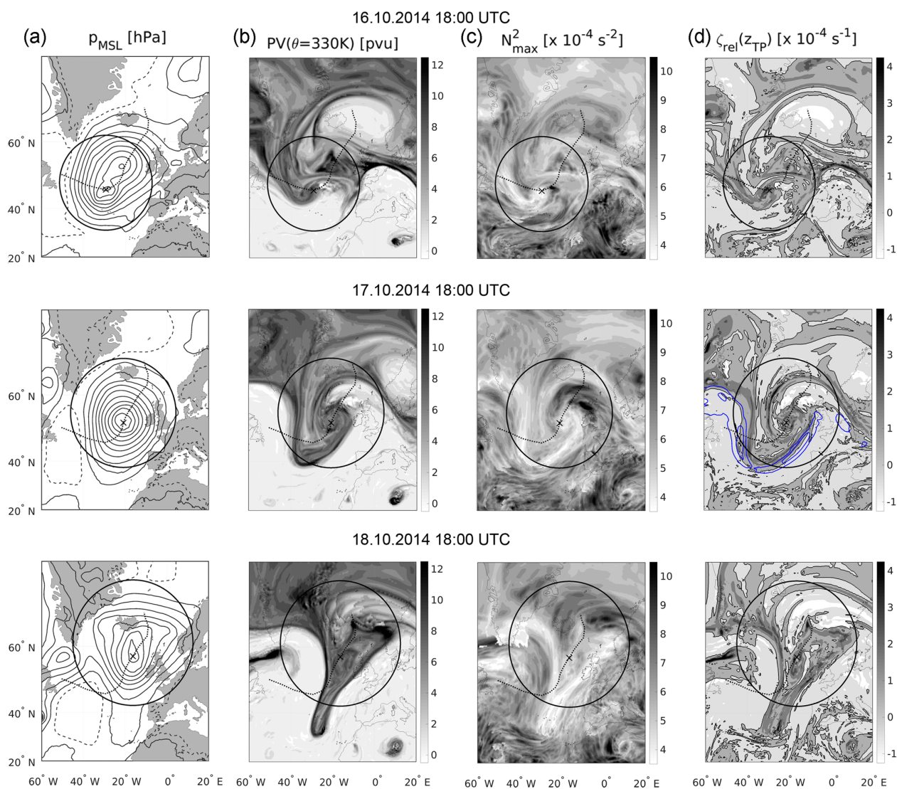
Figure 5. As in Fig. 3, but for the subsequent cyclone with maximum intensity on 17 October 2014 at 18:00 UTC, depicted in the middle row. Top row shows 24 h earlier and bottom row 24 h later.
