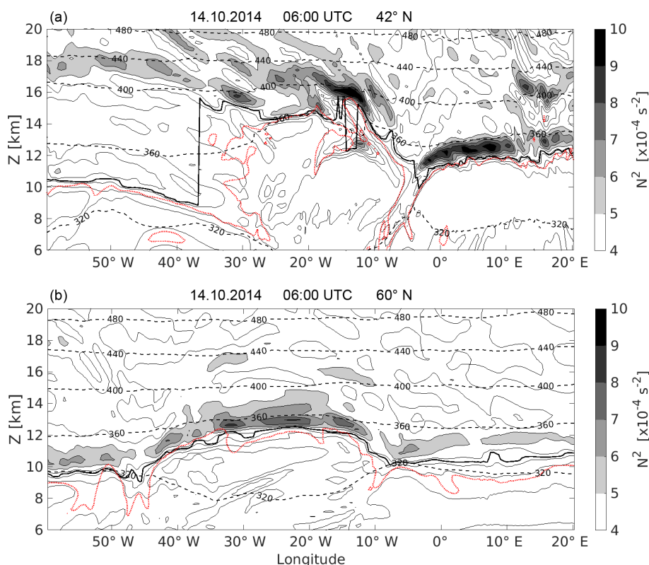
Figure 4. Vertical cross section over the North Atlantic on 14 October 2014 at 06:00 UTC (a) at 42° N and (b) at 60° N. The filled contour as well as the thin solid black contour lines show static stability N^2 in steps of 1 \times 10^{-4} \text{ s}^{-2} , dashed black lines show isentropes. The bold solid black line indicates the lapse rate tropopause, the dotted red line shows the 2 pvu isoline of potential vorticity.
