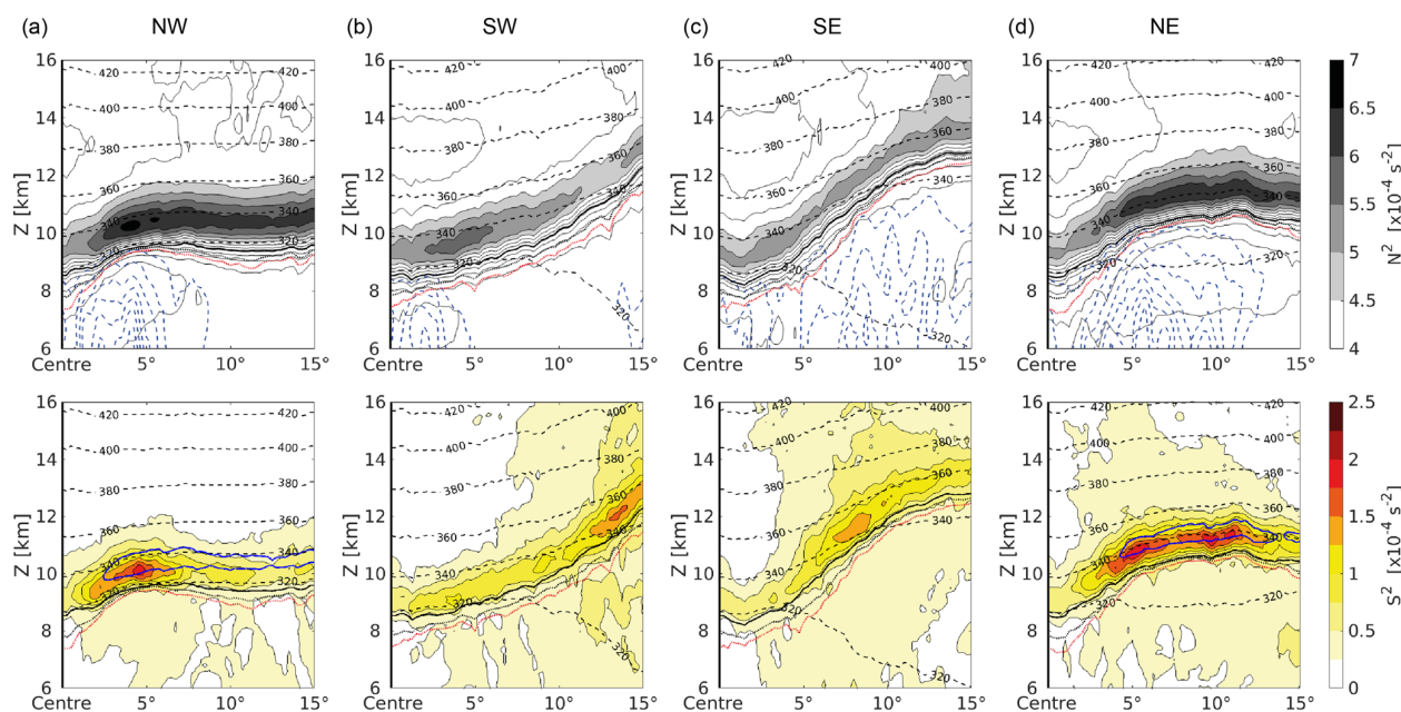
Figure 12. Composites of flow features for the 76 strong cyclones with p_{\text{msl, min}} \leq 990 hPa at the point in time of maximum intensity. Vertical tropopause-based averaged cross section composites, reaching from the cyclone centre (a) northwestward, (b) southwestward, (c) southeastward and (d) northeastward. Top row shows static stability N^2 and cloud ice water content as in Fig. 9, bottom row shows wind shear S^2 as in Fig. 10b. The orientation of the vertical cross sections is indicated by the black arrows in Fig. 11.
