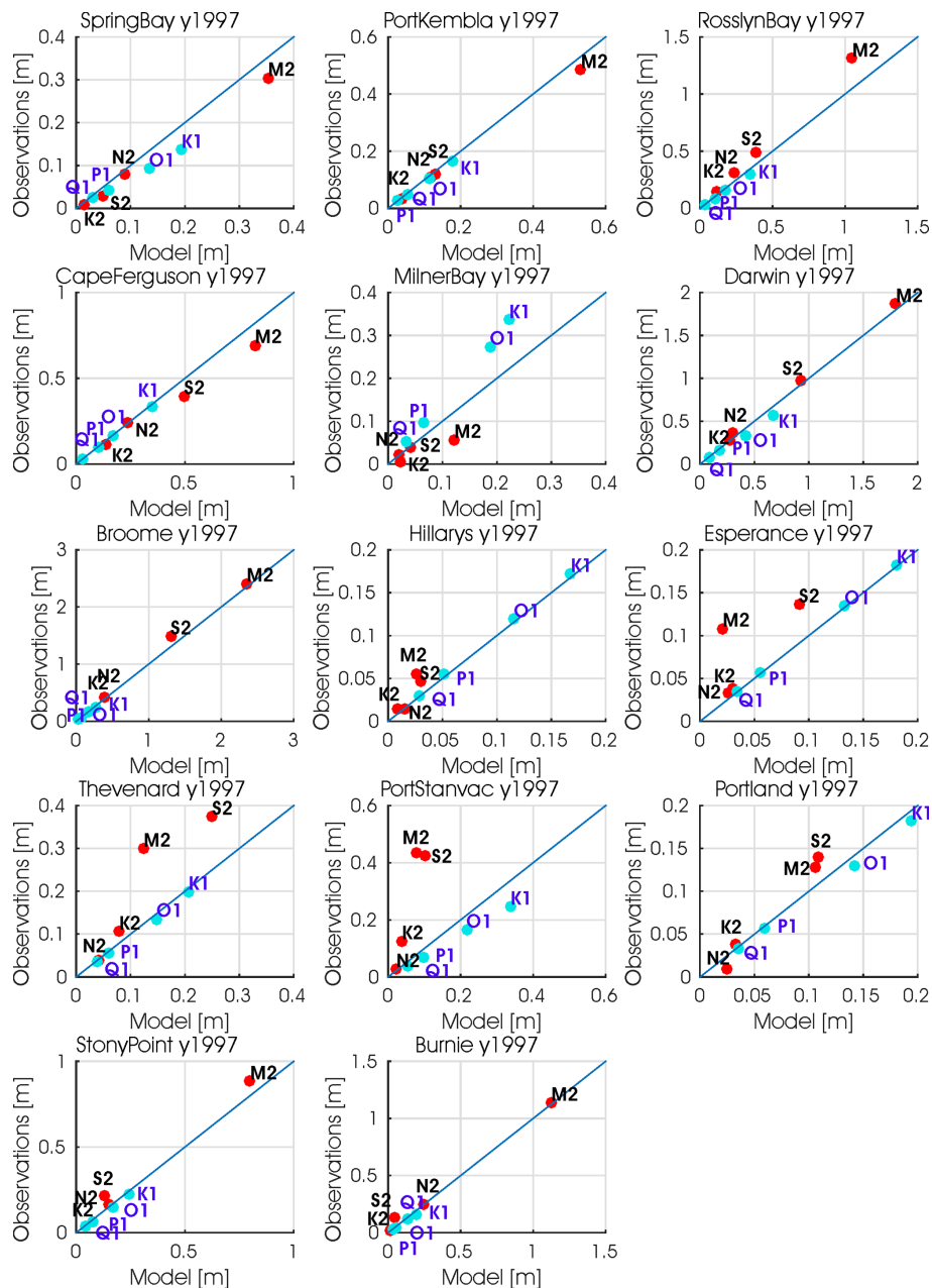
Figure 2. Comparison of the eight major tidal constituents estimated from observations and modelled for the tide gauge locations shown in Fig. 1. Red (blue) dots denote the semi-diurnal (diurnal) tidal constituents respectively.
