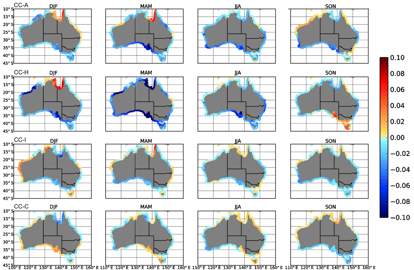
Figure 9. Difference in the average of the seasonal maximum sea level between 2081–2100 and 1981–1999 for the different CC models and seasons indicated. Units are in metres.
