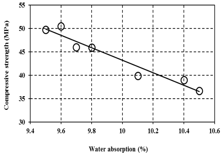
Fig 17. Correlation between water absorption and compressive strength of SCRMs made with various limestone powder contents at age of 28 days.
