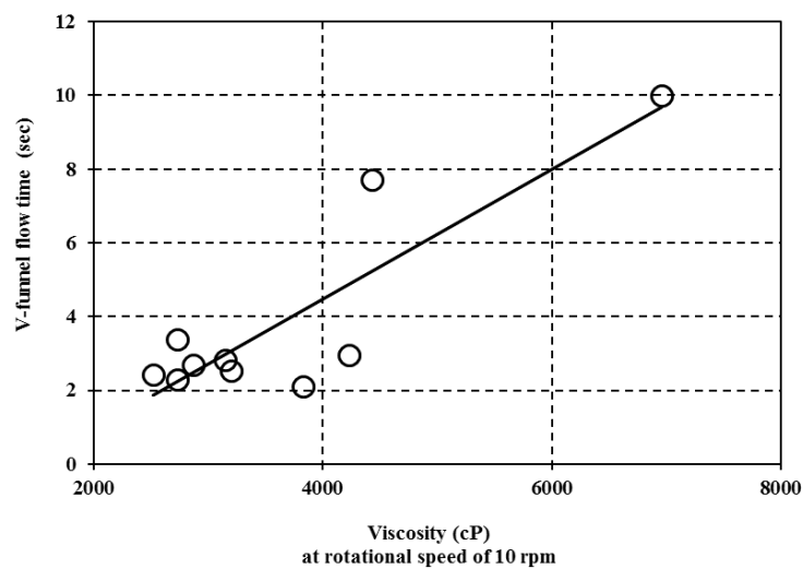
Fig 10. Relationship between V-funnel flow time and viscosity of SCRM.
