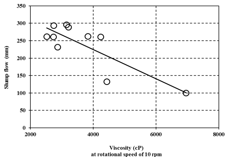
Fig 11. Relationship between slump flow and viscosity of SCRM.
