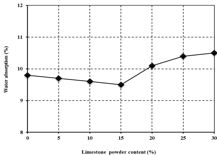
Fig 16. Water absorption percentages of SCRM made of various limestone powder contents at age of 28 days.
