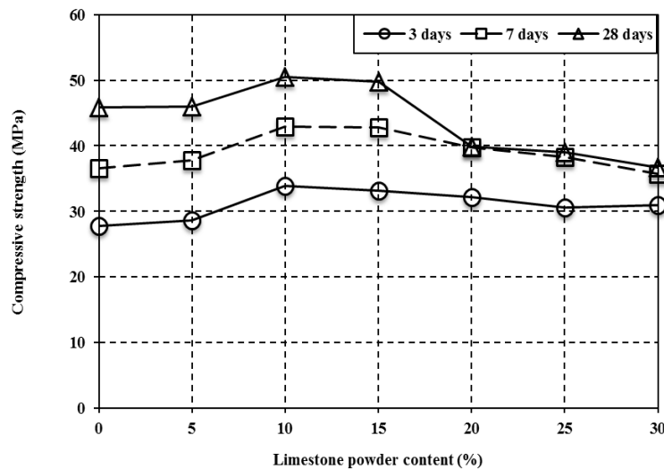
Fig 12. Compressive strength at 3, 7 and 28 days of SCRM made with various limestone powder contents.
