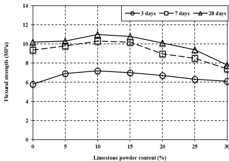
Fig 13. Flexural strength at 3, 7 and 28 days of SCRM made with various limestone powder contents.
