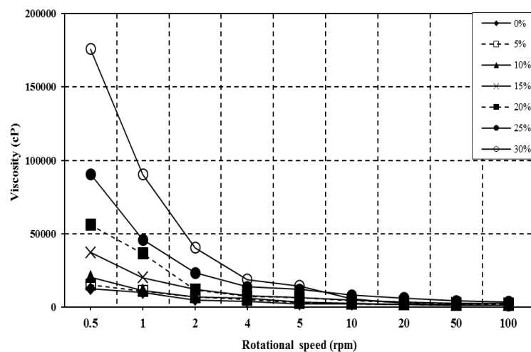
Fig 8. Viscosity of SCRМ with various limestone powder contents at different rotational speeds.
