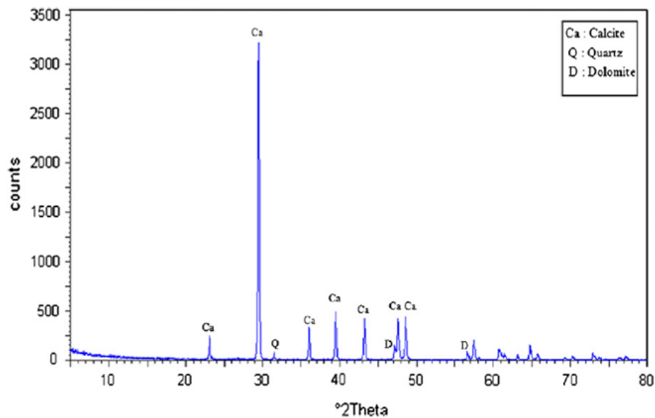
Fig 1. X-ray diffraction of limestone powder.
