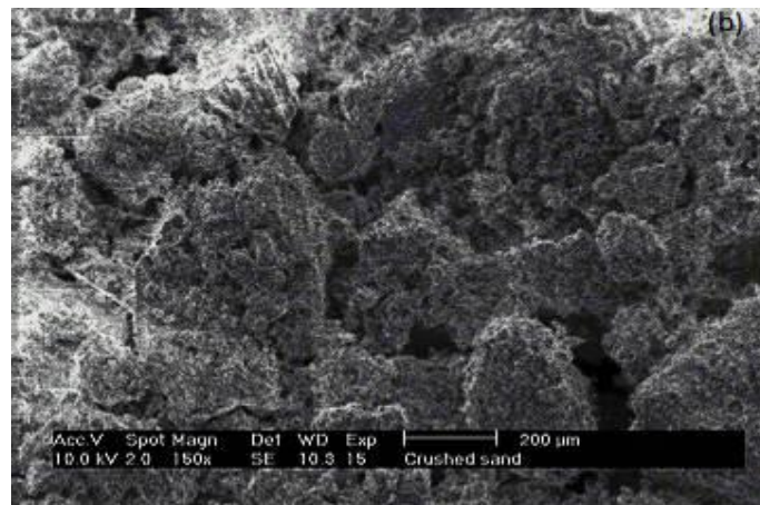
Fig 3. Angular shape of crushed sand grains in SEM view.
