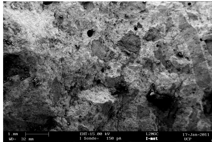
Fig 15. SEM view of hardened SCRM containing 15% of limestone powder at age of 28 days.
