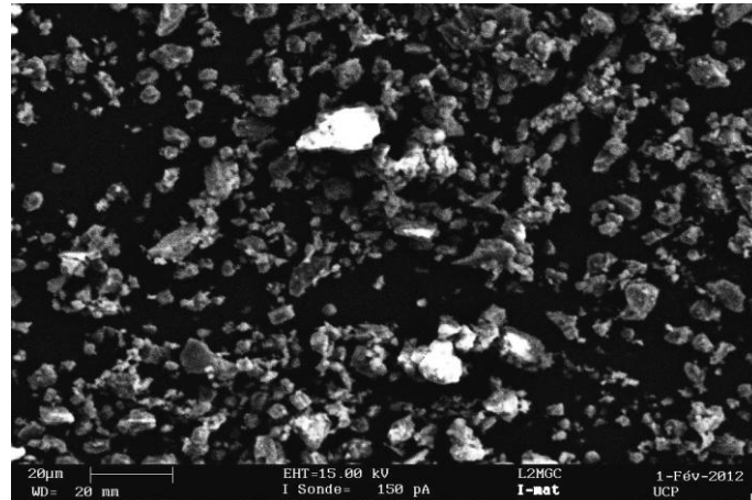
Fig 2. SEM of limestone powder.
