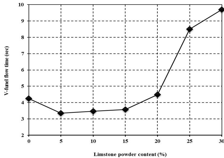
Fig 7. V-funnel flow time test of SCRМ made with various limestone powder contents.
