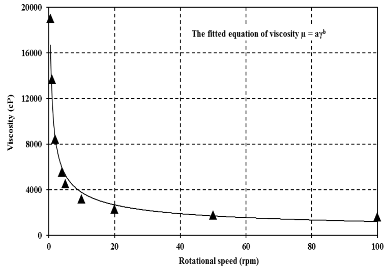
Fig 9. The fitted equation curve of viscosity of SCRM at different rotational speeds.
