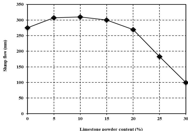
Fig 6. Slump flow test of SCRM made with various limestone powder contents.
