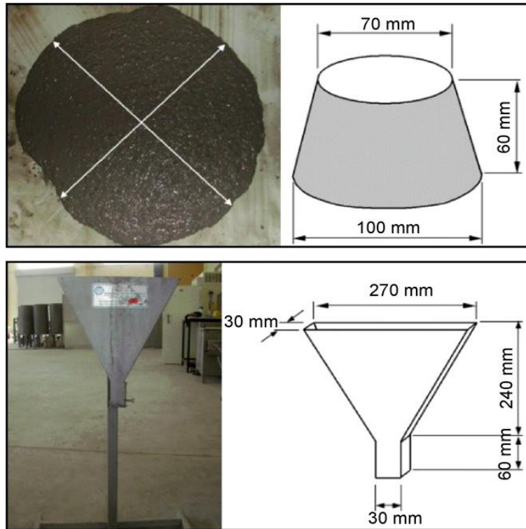
Fig 4. Typical dimensions of mini-spread flow cone and mini-V-funnel apparatus (Felekoğlu et al., 2006).
