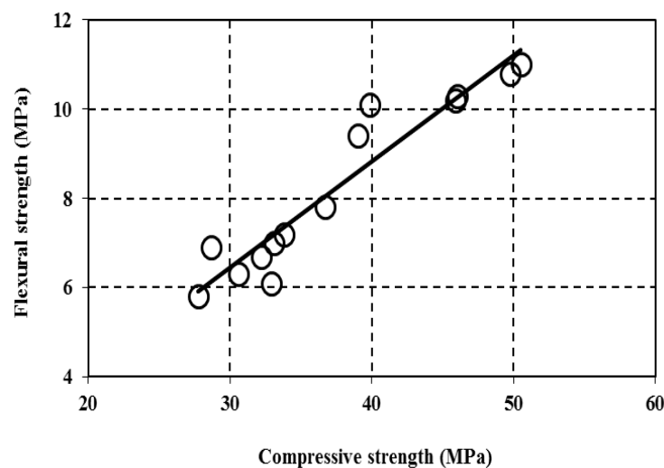
Fig 14. Correlation between flexural and compressive strength of SCRM made with various limestone powder contents at all ages.
