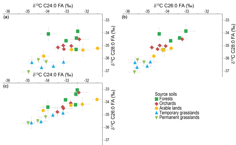
Figure 3. \delta^{13}\text{C} of the FAs (a) C24:0 vs. C28:0, (b) C26:0 vs. C28:0 and (c) C24:0 vs. C26:0 in soils. Error bars: standard deviation of the triplicate measurements.
