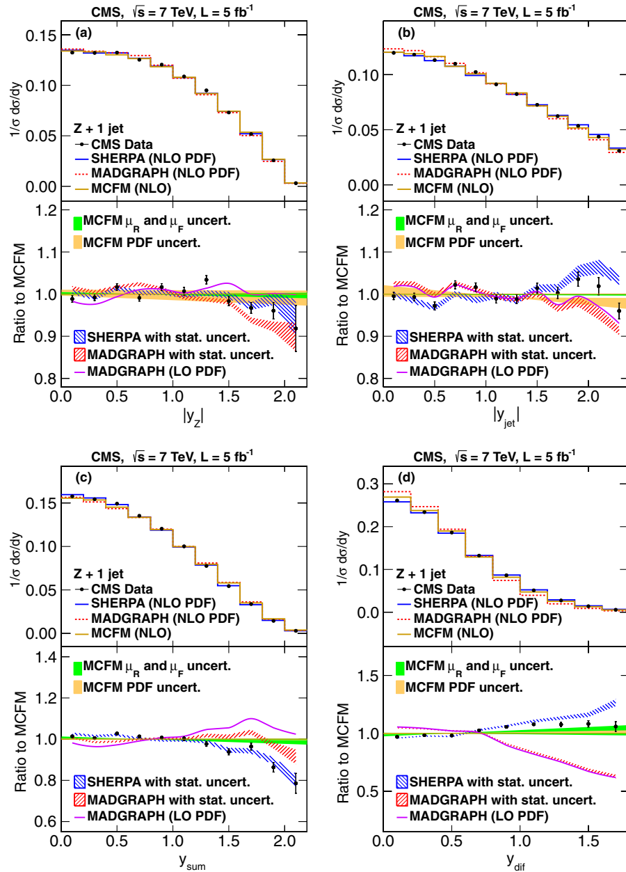
FIG. 1 (color online). Distributions in absolute values of rapidities for (a) the Z boson, (b) the jet, (c) their sums, and (d) their differences, normalized to unity. The data are shown after correcting for efficiency and resolution, and displayed with statistical and systematic uncertainties combined in quadrature. The lower panel of each figure gives ratios of the data and simulations to the NLO calculation of MCFM. The ratio error bars include MCFM statistical uncertainties folded with data statistical and systematic uncertainties. Theoretical uncertainties in the MCFM calculations are shown as shaded areas representing variations of \mu_R , \mu_F , and PDF. Statistical uncertainties for the MADGRAPH and SHERPA predictions are displayed as bands around the central values. The central value for MADGRAPH simulations using LO PDF is depicted by a line. All other calculations use NLO versions of PDF.
