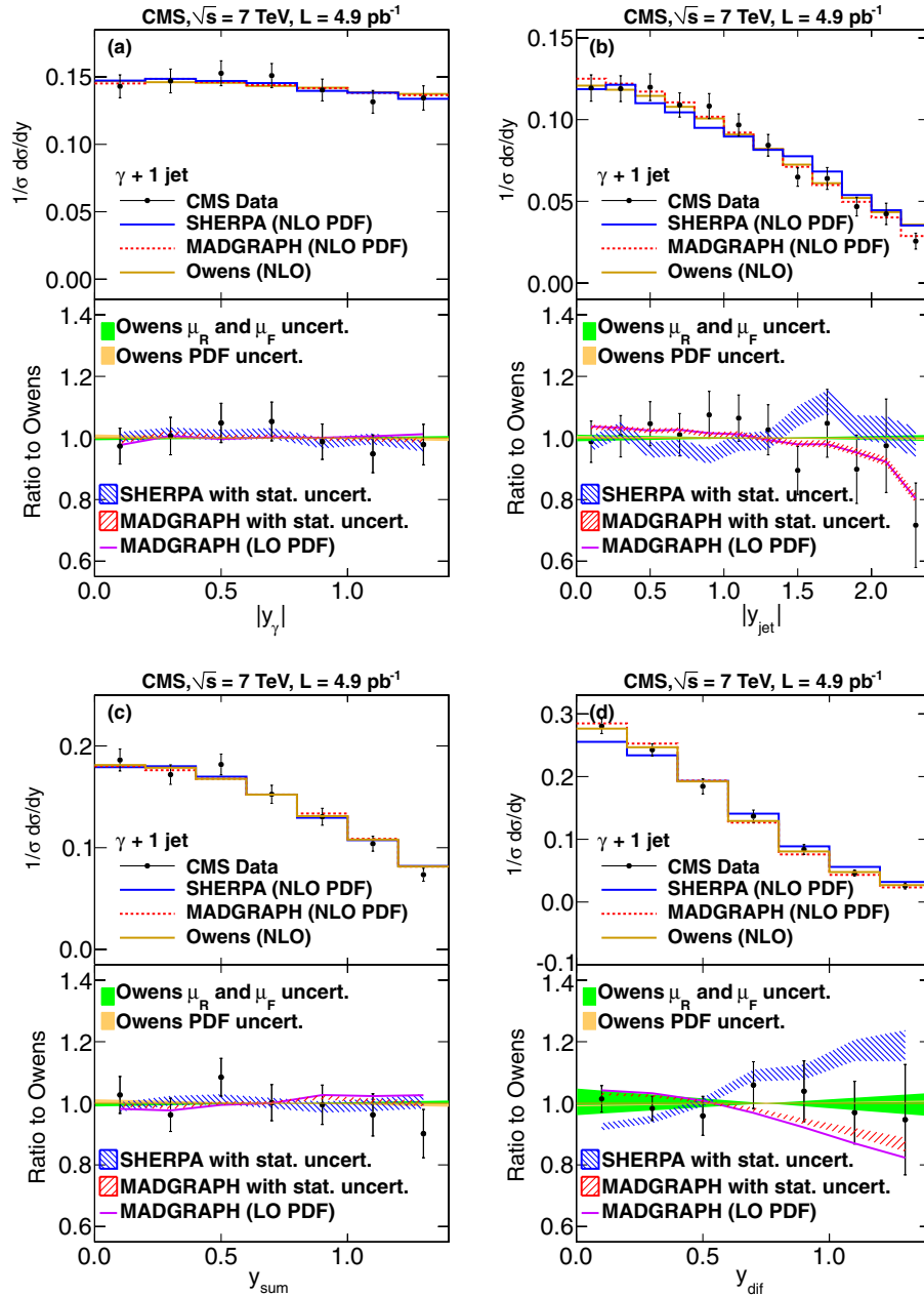
FIG. 2 (color online). Distributions in absolute values of rapidities for (a) the photon, (b) the jet, (c) their sums, and (d) their differences, normalized to unity. The data are shown after correcting for efficiency and resolution, and displayed with statistical and systematic uncertainties combined in quadrature. The lower panel of each figure gives ratios of the data and simulations to the NLO calculation of Owens. The ratio error bars include Owens statistical uncertainties folded with data statistical and systematic uncertainties. Theoretical uncertainties in the Owens calculations are shown as shaded areas representing variations of \mu_R , \mu_F , and PDF. Statistical uncertainties for the MADGRAPH and SHERPA predictions are displayed as bands around the central values. The central value for MADGRAPH simulations using LO PDF is depicted by a line. All other calculations use NLO versions of PDF.
