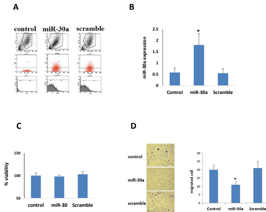
Figure 1. A. Evaluation of transfected melanoma cell with flow cytometry; over 75% of cells have been transfected by miR-30a-5p and scramble. B. Real-time PCR of miR-3a-5p in B16F10 melanoma cell lines after transfection with miR-30a-5p and scramble in comparison with control. C. MTT analysis showed that both miR-30a-5p and scramble have no obvious effects on viability of melanoma cells. D. Image and histogram of cell migration evaluated by Boyden chamber.*, P < 0.05 compared to the control and scramble groups
