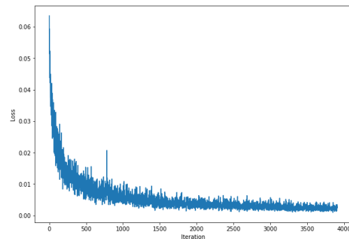
Fig. 16. Loss vs iteration graph while training face95
