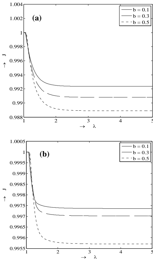
Fig. 8. Radiation profiles for Royce EOS when \Gamma_0 = 1.4 , \sigma = 1.42 ; (a) \Omega = 2 and (b) \Omega = 3
