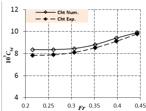
Fig. 15. Experimental and computational hull resistance coefficient in surface condition
