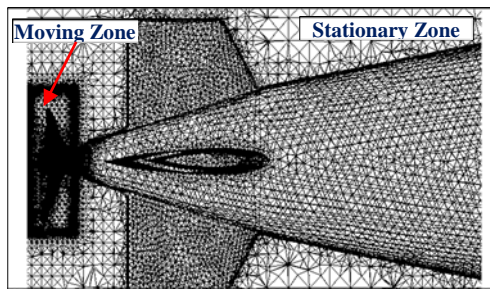
Fig. 8. Generated grid around the propeller and at the back of the submarine; side view
