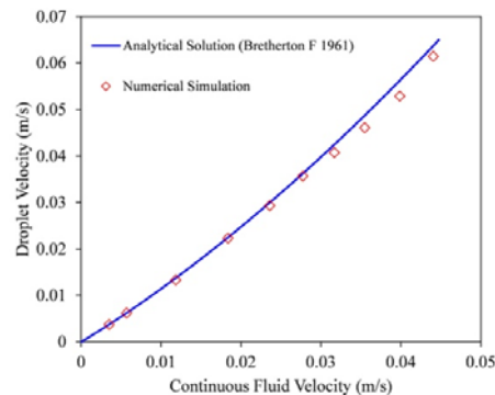
Fig. 4. Droplet velocity of a long droplet as a function of mean velocity of the carrier fluid in a tube. Comparison of the numerical simulation results with the Bretherton (1961) analytical relation shows the numerical results is acceptable.
