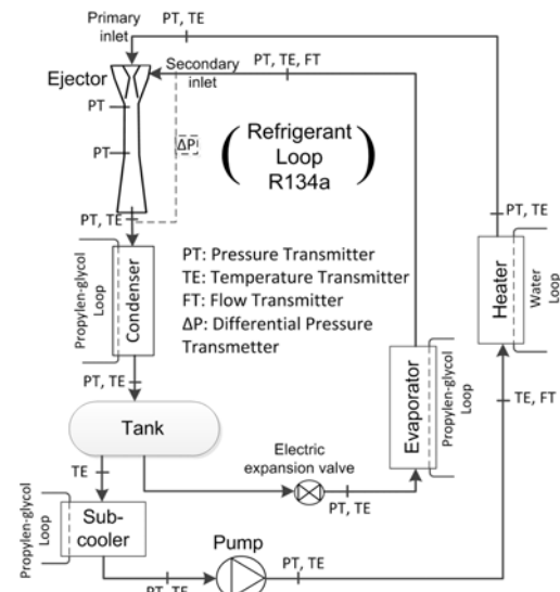
Fig. 3. Diagram of the test rig.
