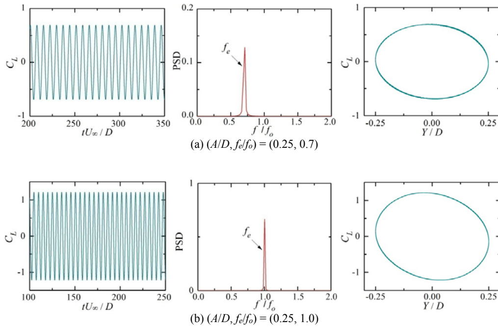
Fig. 2. Time evolutions of the lift coefficient C_L (left column), power spectral density (PSD) of the lift coefficient (middle column) and phase portraits for the oscillating cylinder at: (a) (A/D, f_e/f_o) = (0.25, 0.7) ; (b) (A/D, f_e/f_o) = (0.25, 1.0) .
