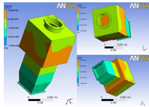
Fig. 12. Distribution of pressure for the plenum chamber.
